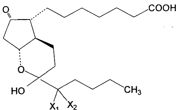
Tautomer II
