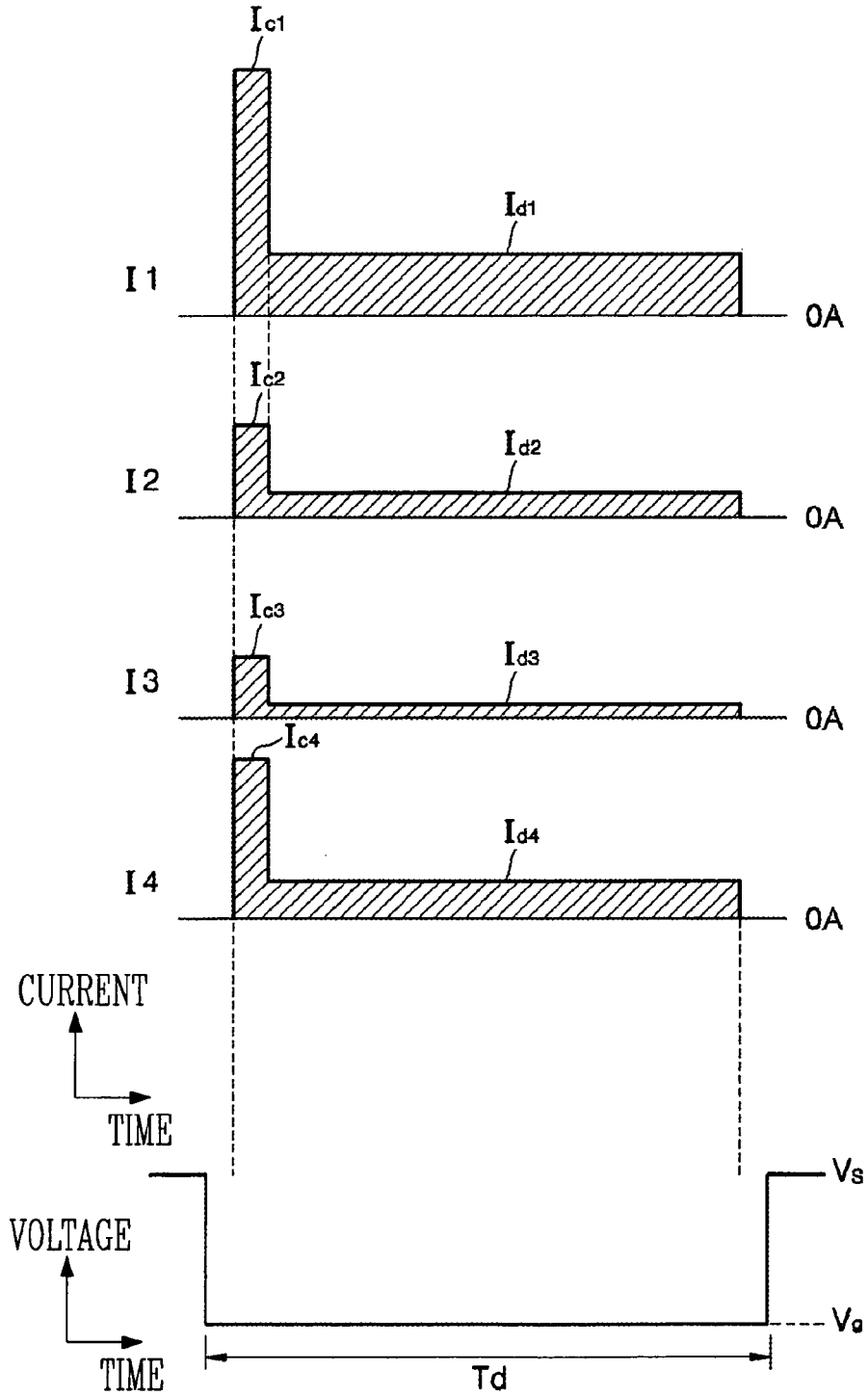
FIG. 4 (Prior Art)
