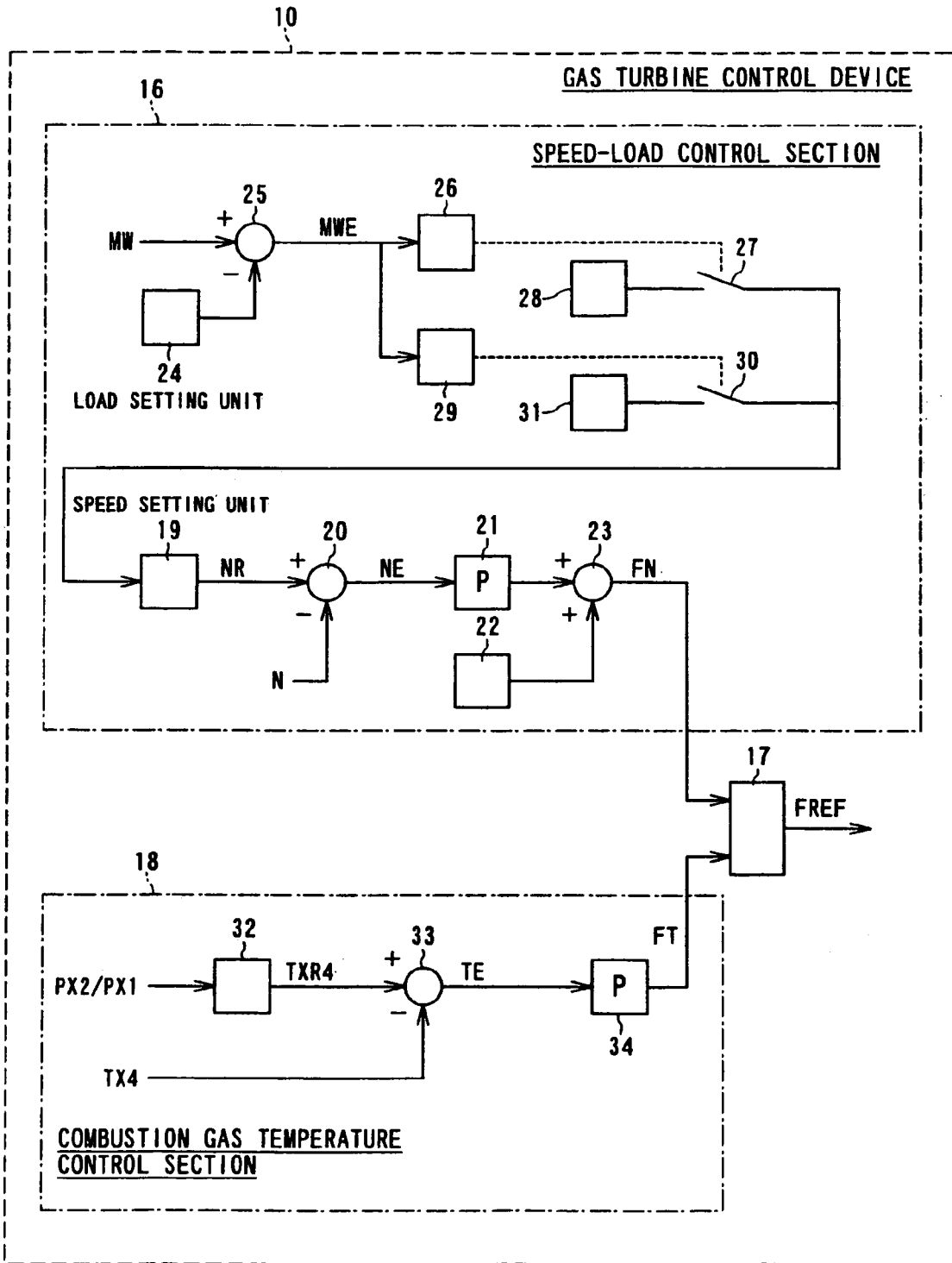
FIG. 37 PRIOR ART
