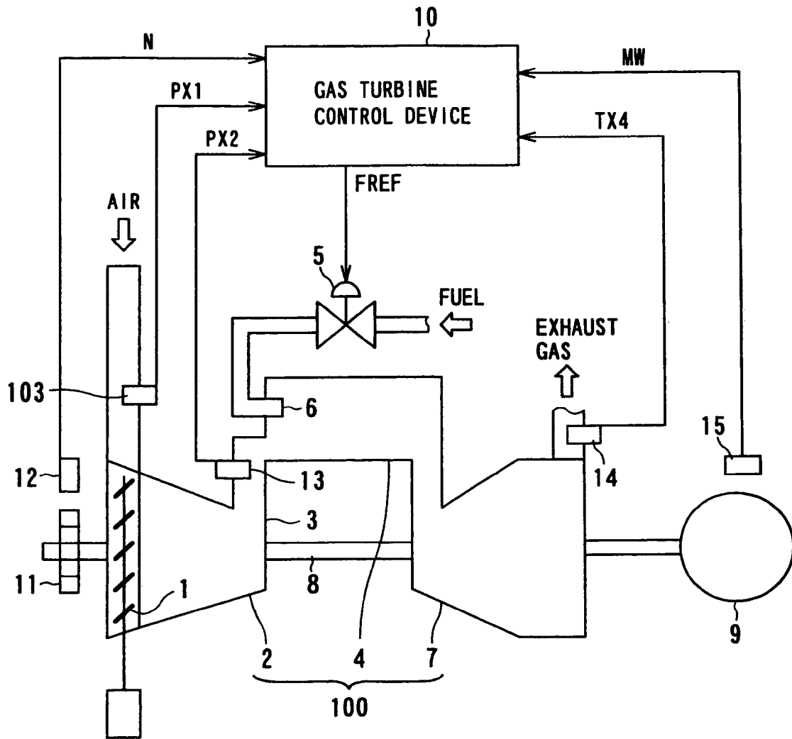
FIG. 36 PRIOR ART
