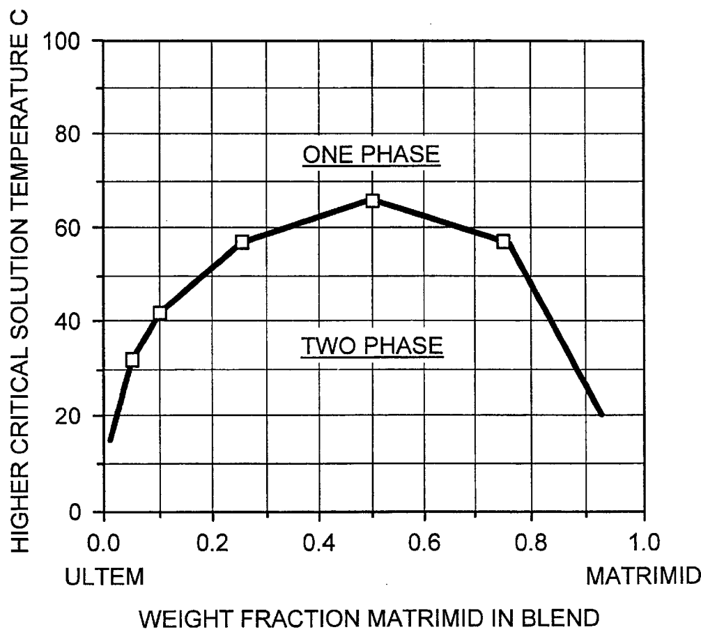
Coexistence Curve for ULTEM/MATRIMID Blends (31% Total Polymer Content in NMP)
