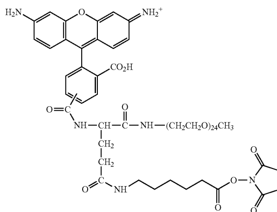
Compound No. 77
