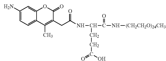
Compound No. 78
