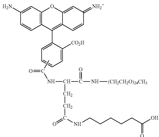
Compound No. 76
