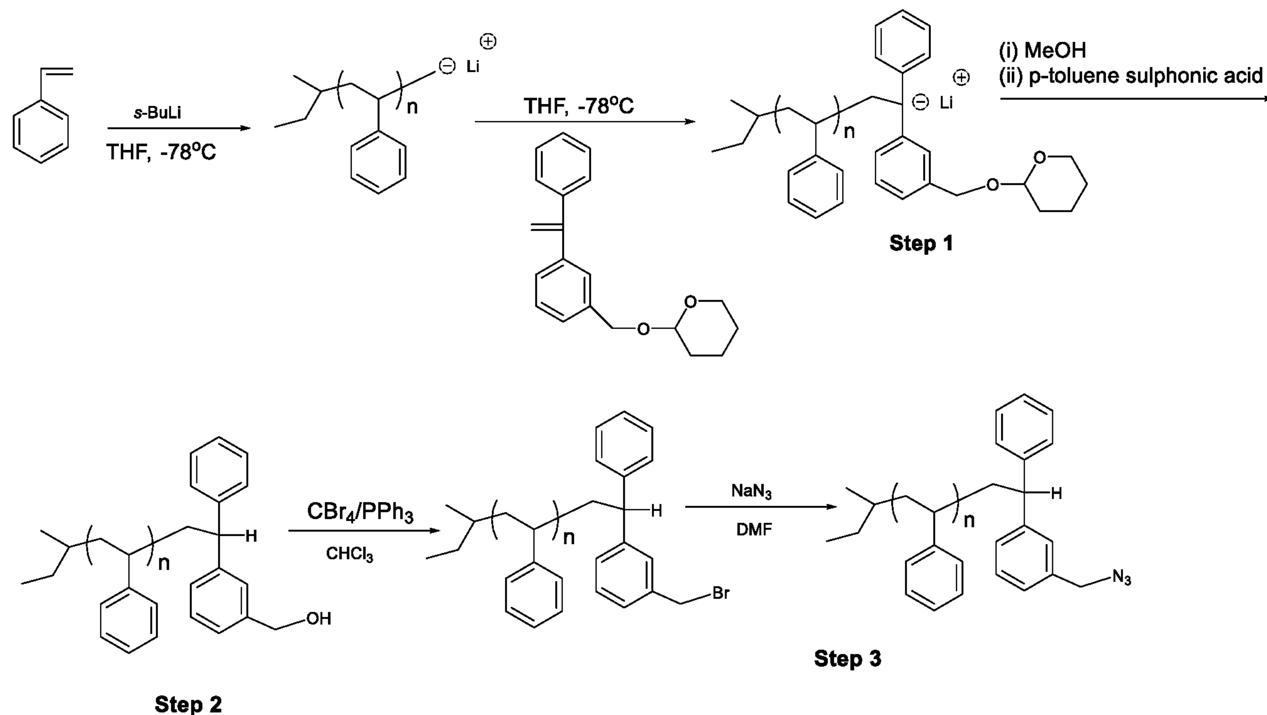
Scheme 1: Synthesis of azide terminated polystyrene
