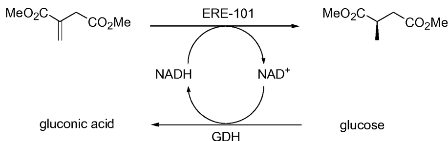
Scheme 4. Reaction scheme.
