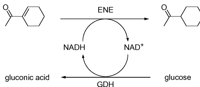
Scheme 3. Reaction scheme.
