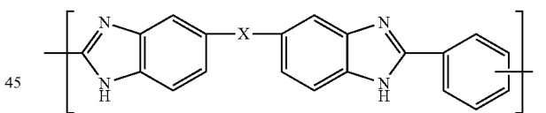
[Chemical Formula 2]
