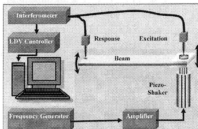
Setup of the Laser-Doppler-Vibrometer Method
