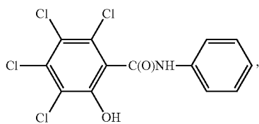
tetrachlorosalicylanilide
