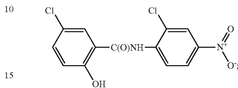
niclosamide
