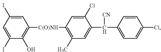
closantel
