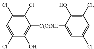
oxyclozanide
