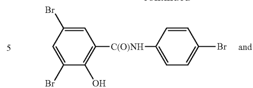
tribromosalalan
