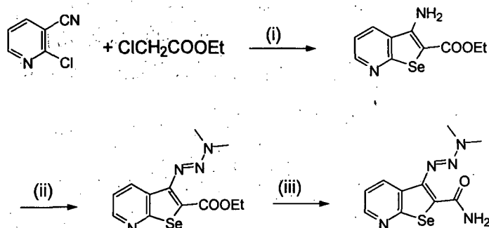
Compound 6
