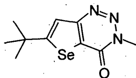
compound 13
