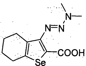
compound 9
