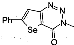
compound 12
