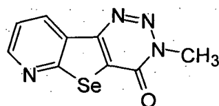
compound 15
