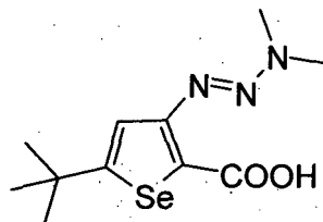
compound 8
