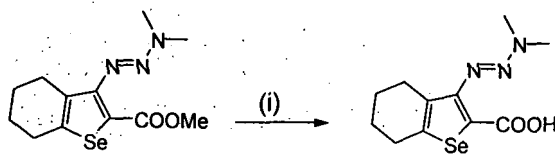
Compound 9
