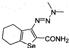
compound 5
