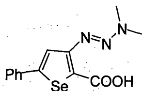
compound 7
