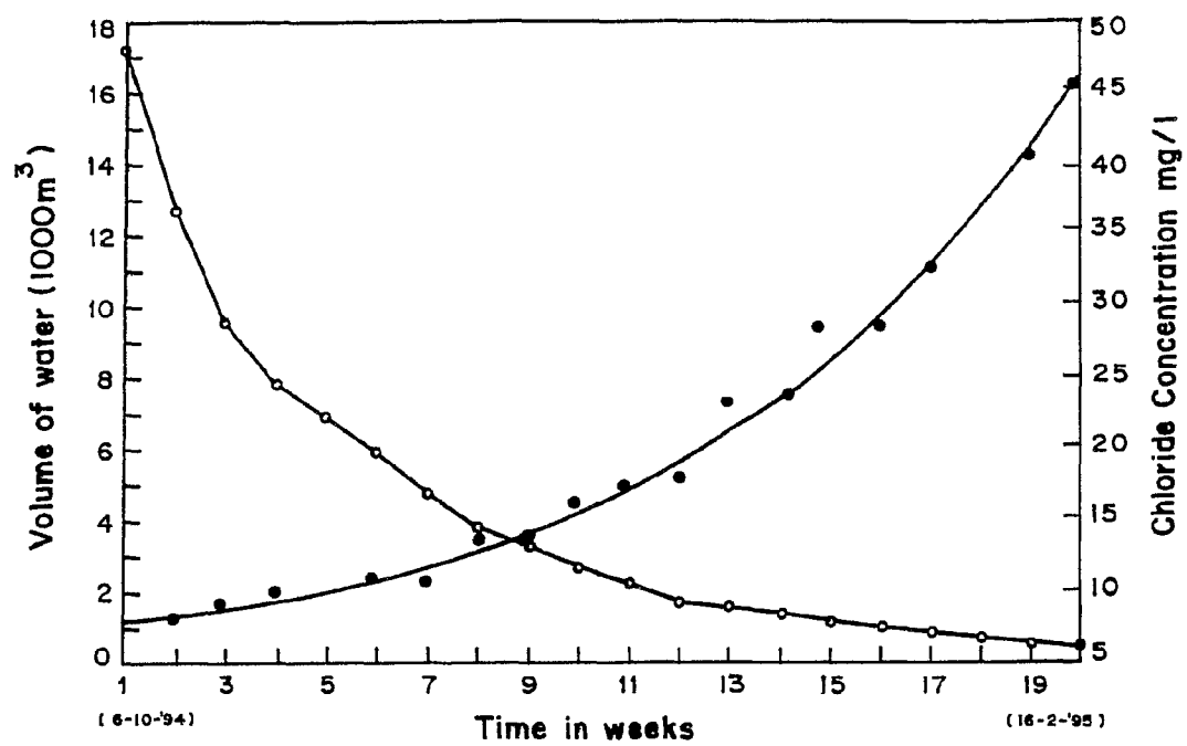
Fig.2: Temporal variation of volume of water and its chloride concentration in percolation tank
