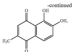
(6-hydroxyplumbagin)
