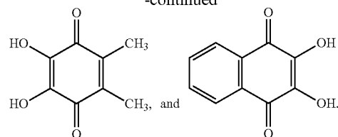
(Isonaphthazin)
