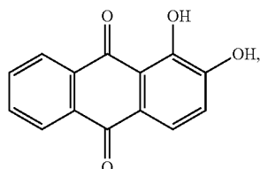
(Alizarin)
