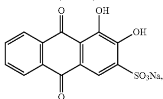
(Alizarin-S)
