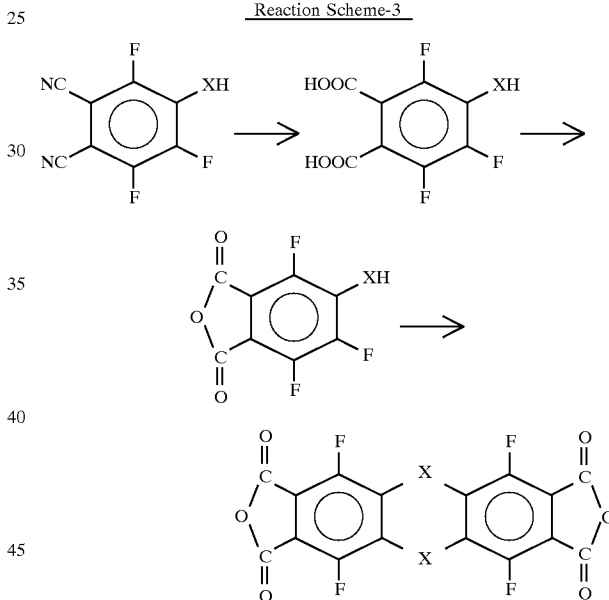
Reaction Scheme-3
