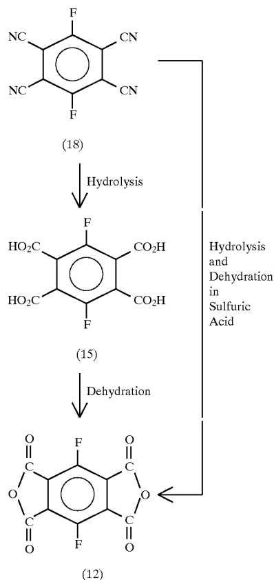
Reaction Scheme-8
