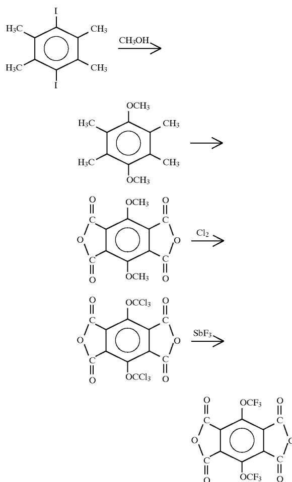
Reaction Scheme-1
