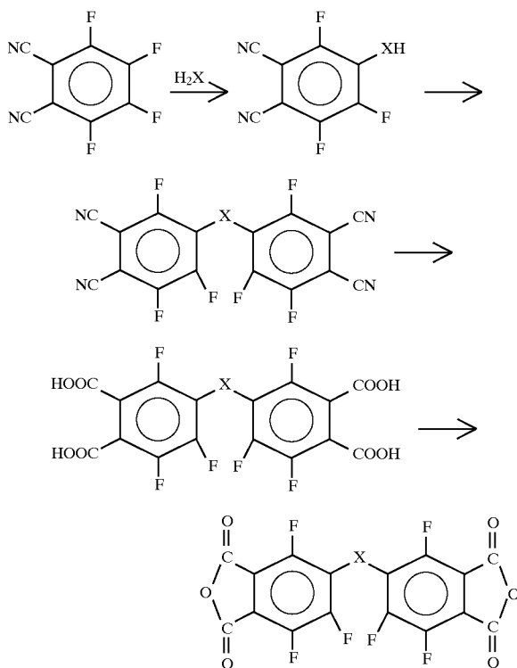
Reaction Scheme-2
