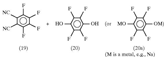
Reaction Scheme-7
