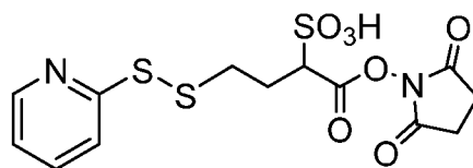
N-succinimidyl-4-(2-pyridyldithio)-2-sulfo-butanoate (sulfo-SPDB).
