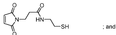
MPET: MaleimidoPropionamidoEthylThio
