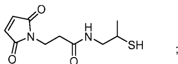
MPPT: MaleimidoPropionamidoPropaneThio
