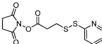
N-succinimidyl-3-(2-pyridyldithio)propionate (SPDP),
