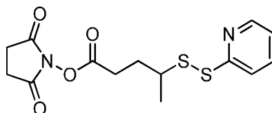
N-succinimidyl-4-(2-pyridyldithio)pentanoate (SPP),
