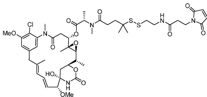
MPET-DM4
