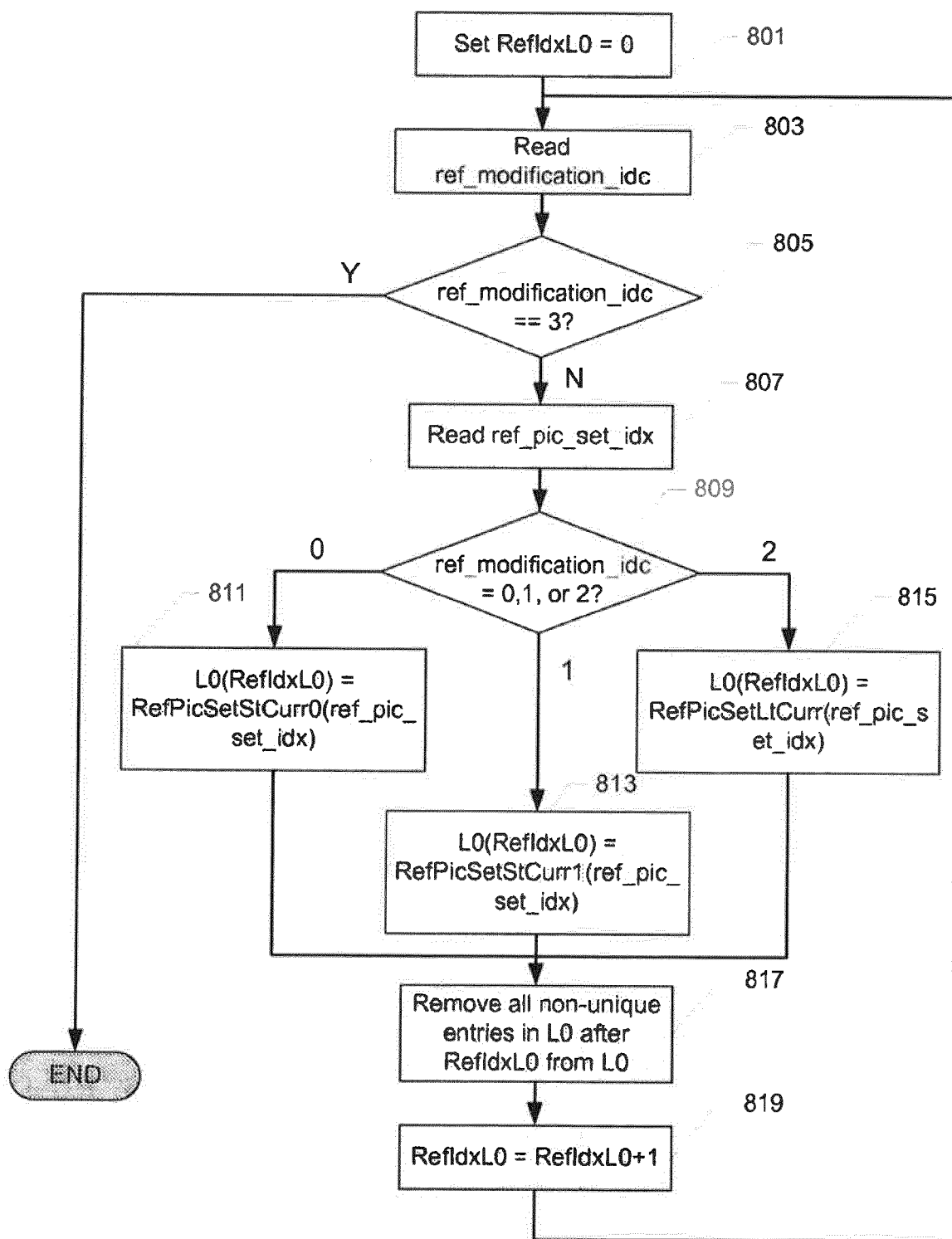
FIG. 8 (PRIOR ART)
