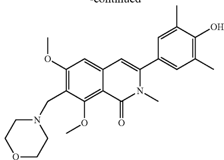
3-(4-hydroxy-3,5-dimethylphenyl)-6,8-dimethoxy-2,7-dimethylisoquinolin-1(2H)-one (left) and 3-(4-hydroxy-3,5-dimethylphenyl)-6,8-dimethoxy-2-methyl-7-(morpholinomethyl)isoquinolin-1(2H)-one (right)
