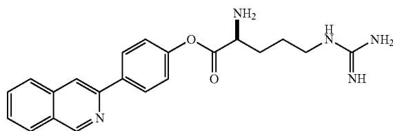
4-(Isoquinolin-3-yl)phenyl 2-amino-5-guanidinopentanoate tetrahydrochloride
