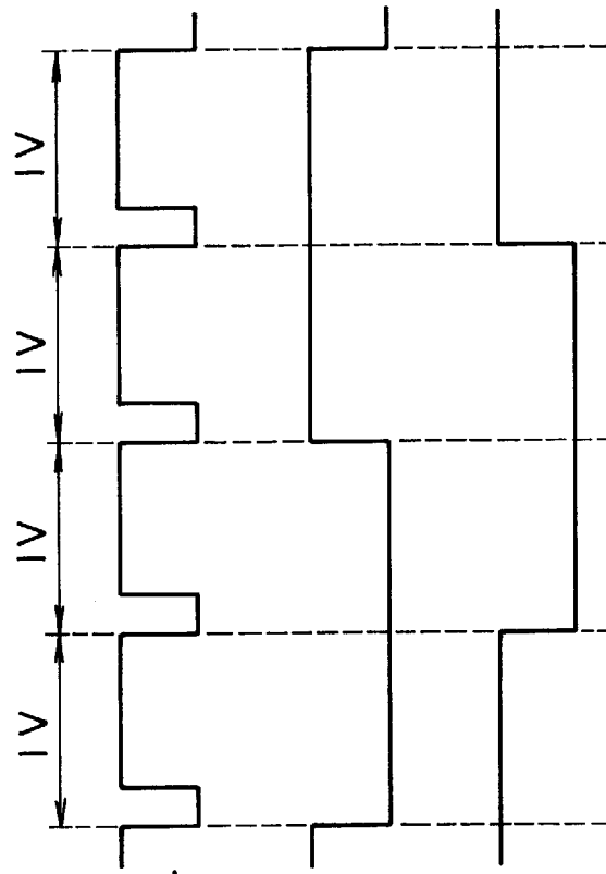
VERTICAL SYNC SIGNAL
