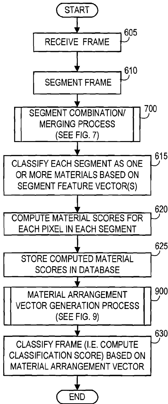
FIG. 6 OUTDOOR CLASSIFICATION
