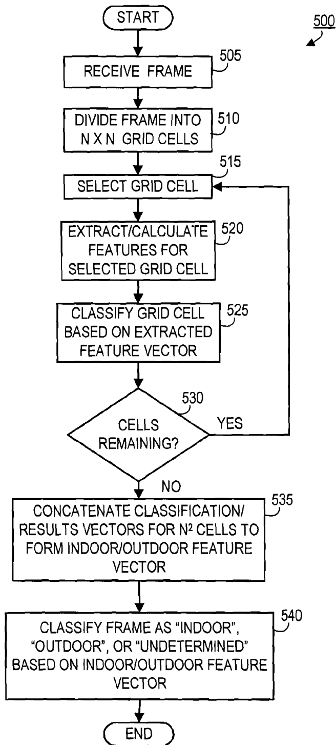
FIG. 5 INDOOR/OUTDOOR CLASSIFICATION
