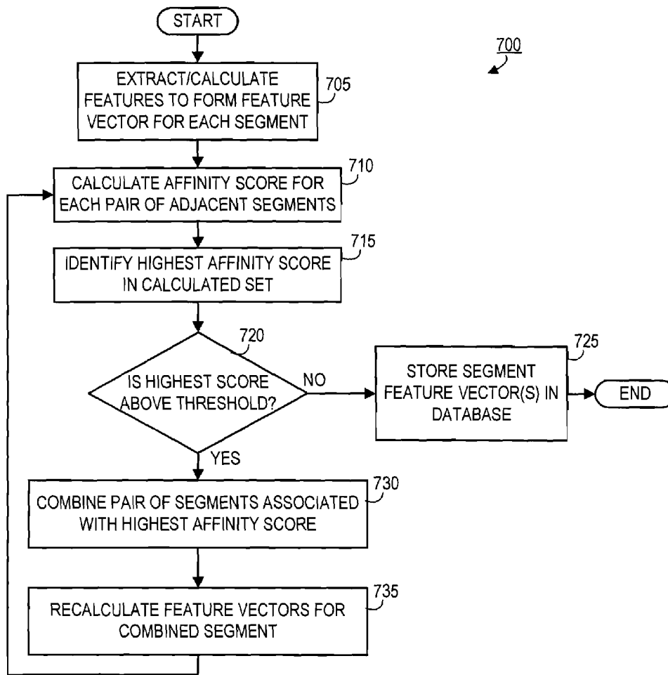
FIG. 7 SEGMENT COMBINATION/MERGING PROCESS
