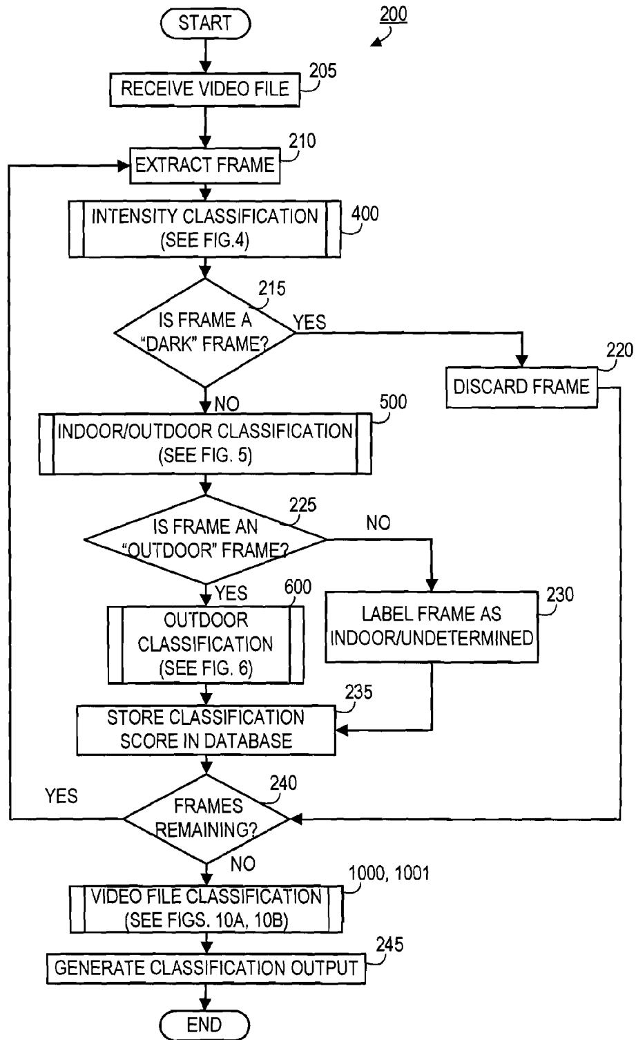
FIG. 2 OVERALL CLASSIFICATION SYSTEM
