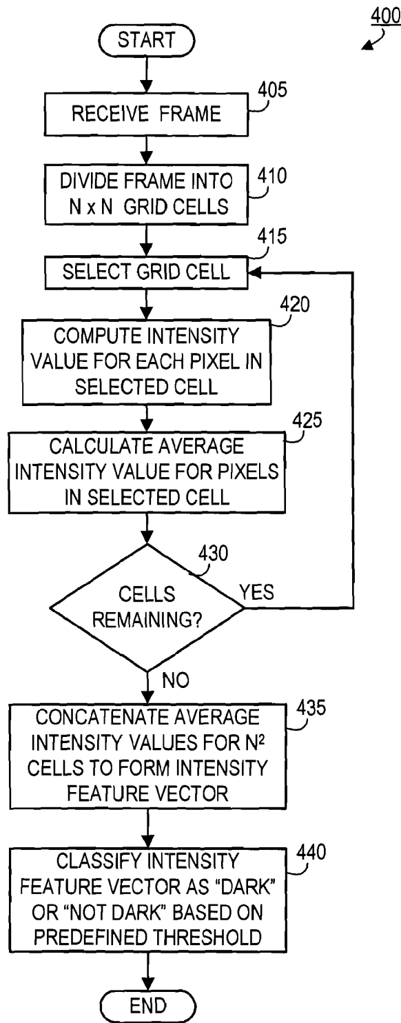
FIG. 4 INTENSITY CLASSIFICATION
