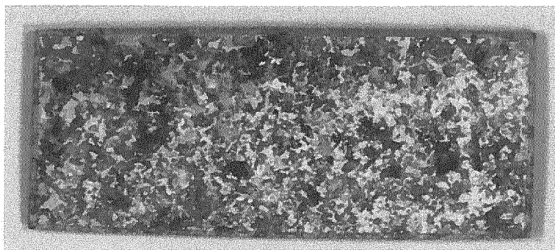
Ti-6Al-2Sn-4Zr-2Mo-0.1Si
