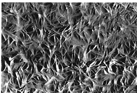
Ti-15Mo-3Nb-3Al-0.3Si
