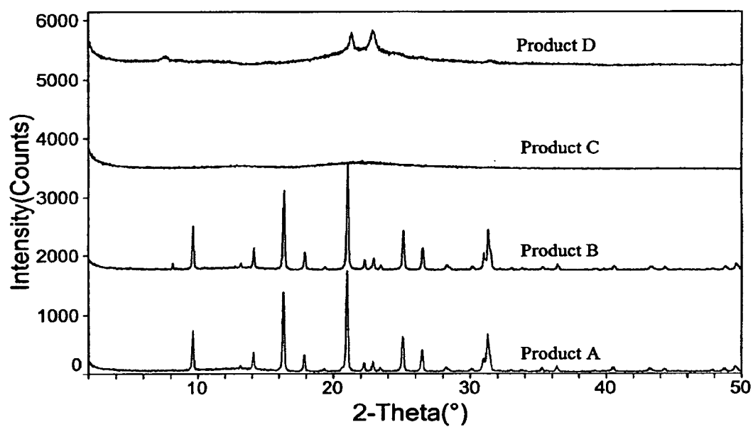
Figure 1. XRD Patterns of Products
