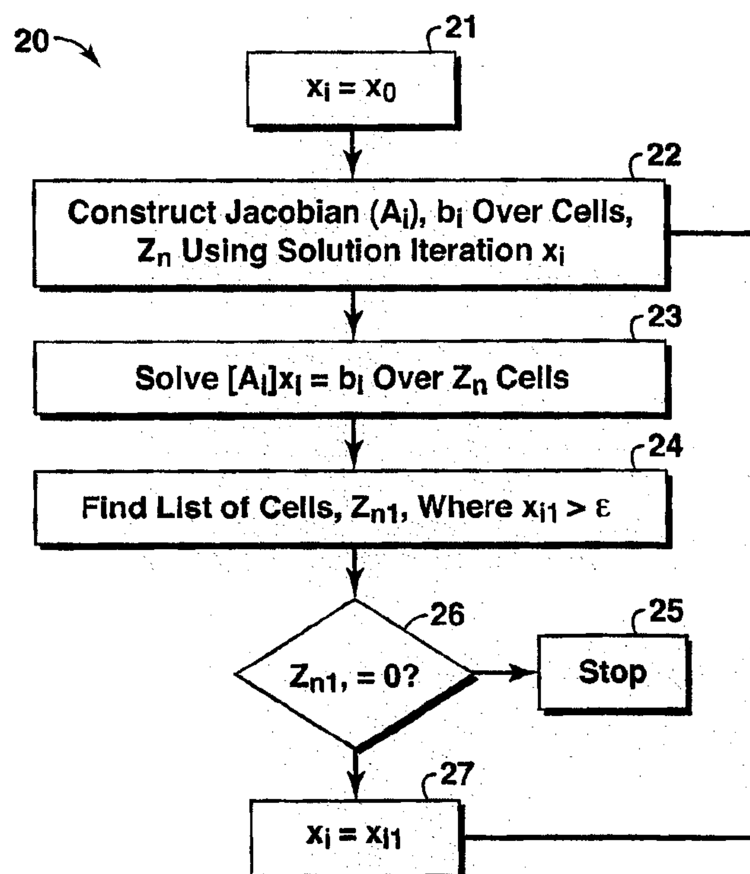
FIG. 2 Prior Art
