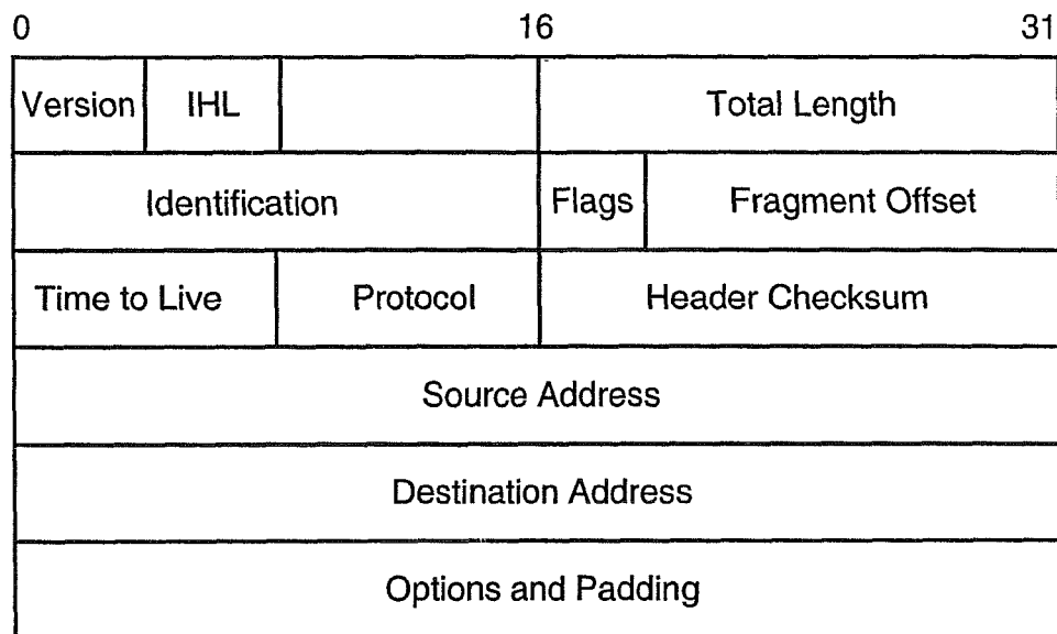
Internet Protocol v.4 Header
