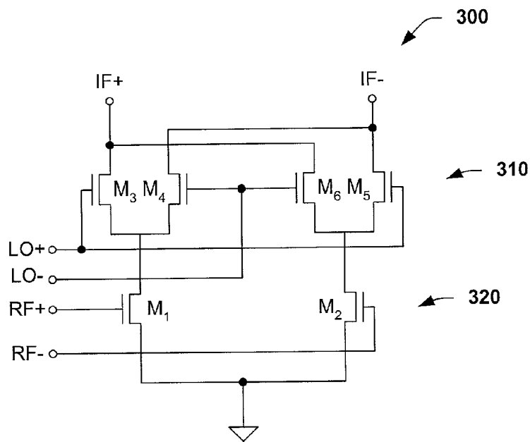
FIG. 5 PRIOR ART
