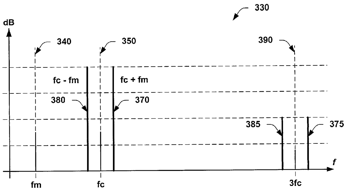
FIG. 5 PRIOR ART
