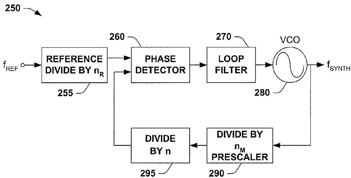
FIG. 3 PRIOR ART
