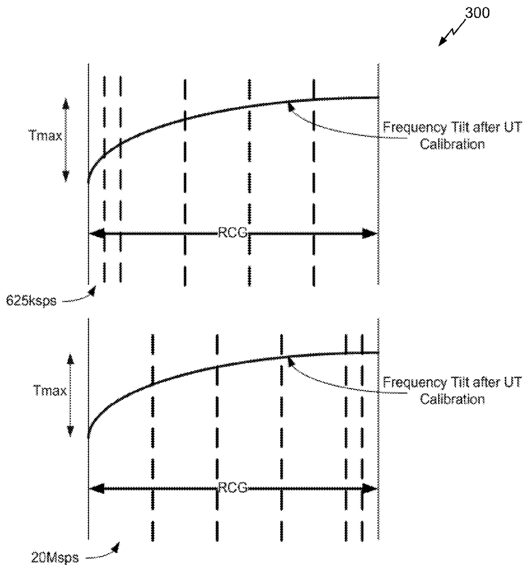
Exemplary channel configurations showing a group of return link channels (Return Channel Group (RCG)) of various symbol rates from 20Msps to 625ksps and showing a frequency-dependent gain at the User Terminal
