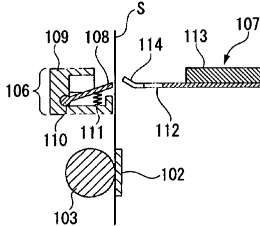
FIG. 7F PRIOR ART
