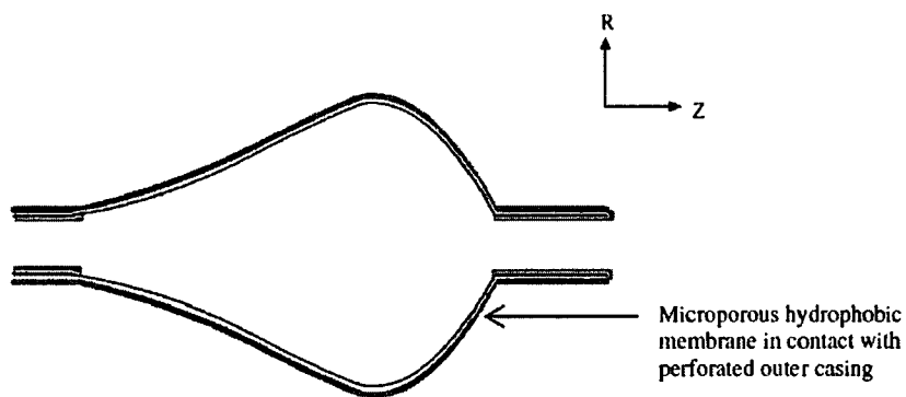
Figure 2: Longitudinal Section of Air Filter with positive internal gauge pressure
