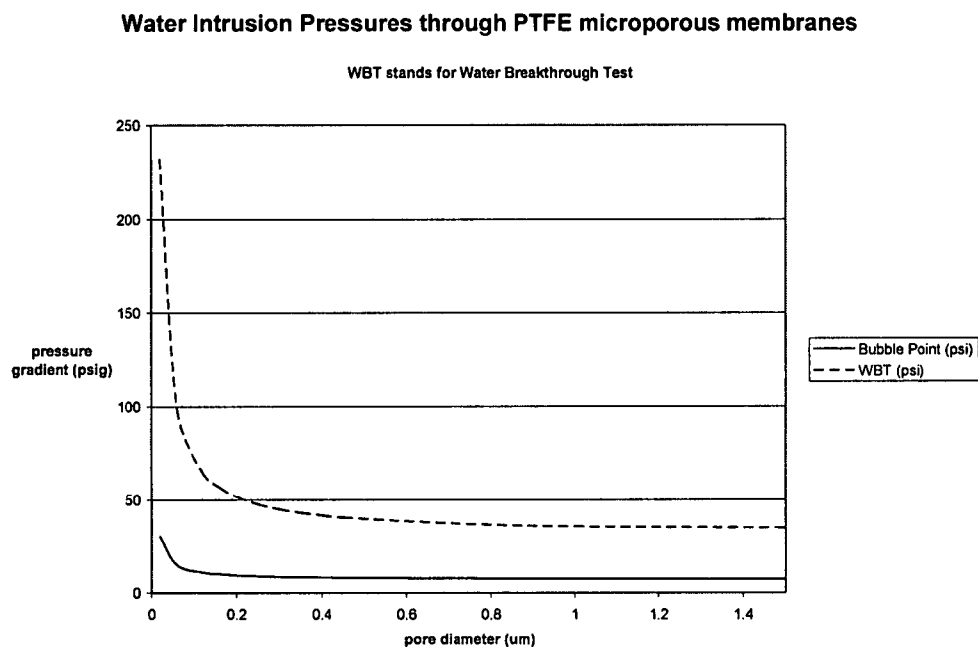
Figure 12: Graph of water intrusion pressures through PTFE membrane
