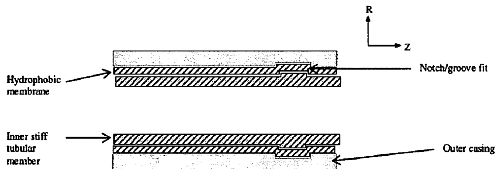
Figure 6: Longitudinal section of joint assembly detail
