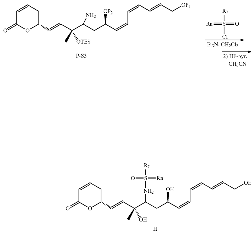
Reaction scheme 5:
