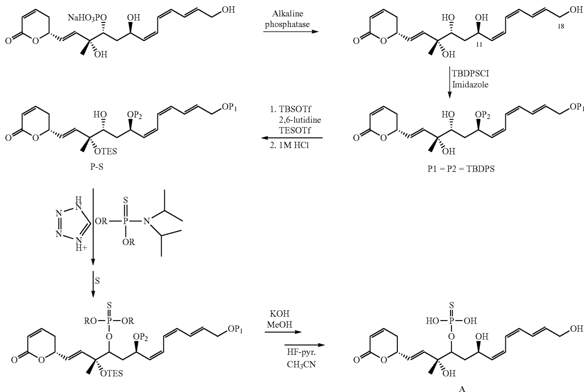
Reaction scheme 1:
