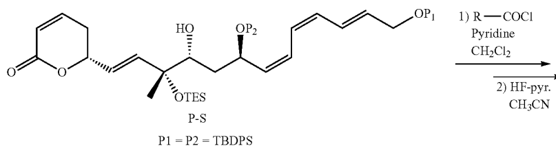
Reaction scheme 3:
