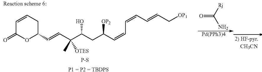
Reaction scheme 6:
