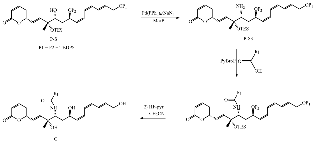
Reaction scheme 4:
