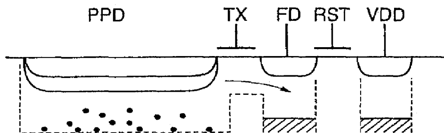
FIG. 1 (PRIOR ART)
