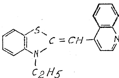
4-[1-cyano-5-(3-methyl-2(3H)-benzothiazolylidene)-1,3-pentadienyl]quinoline
