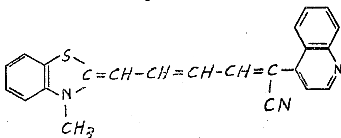
4-[1-cyano-5-(3-methyl-2(3H)-benzothiazolylidene)-1,3-pentadienyl]quinoline
