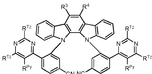
Formula IVa
