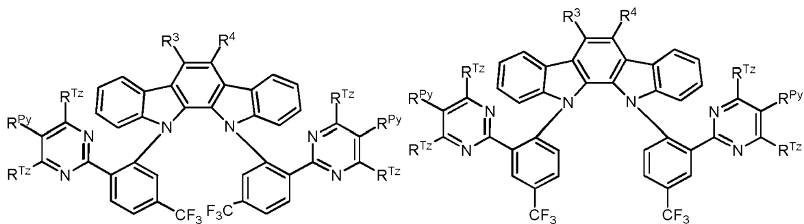
Formula Ve
