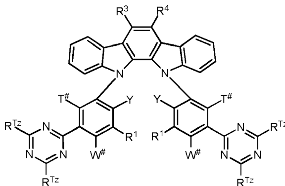
Formula IX
