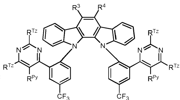
Formula IVf
