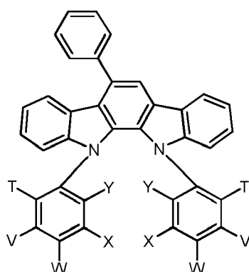
Formula III-AA
