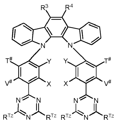
Formula VI
