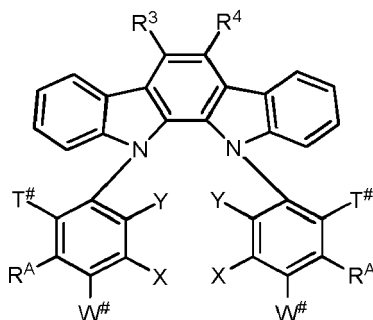
Formula III-YYY
