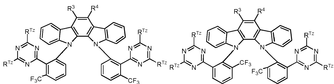
Formula IIIg
