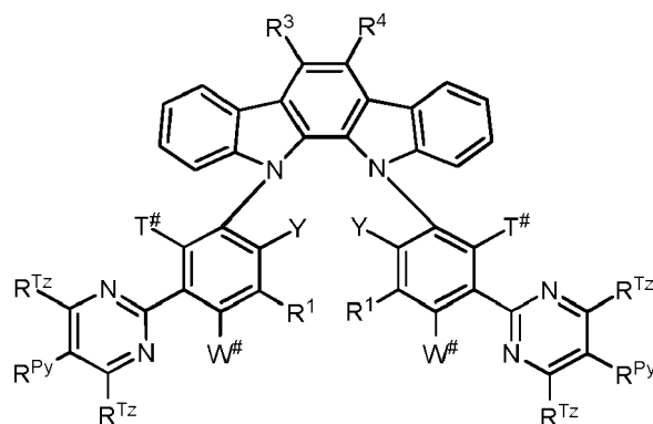
Formula XI
