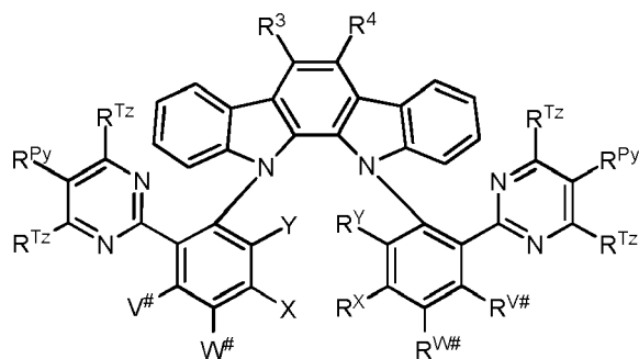
Formula V
