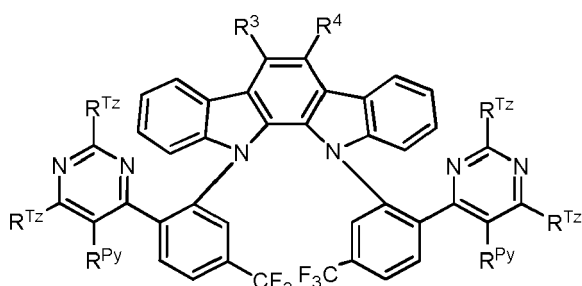
Formula IVe
