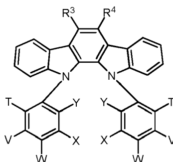
Formula I
