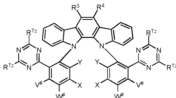
Formula III
