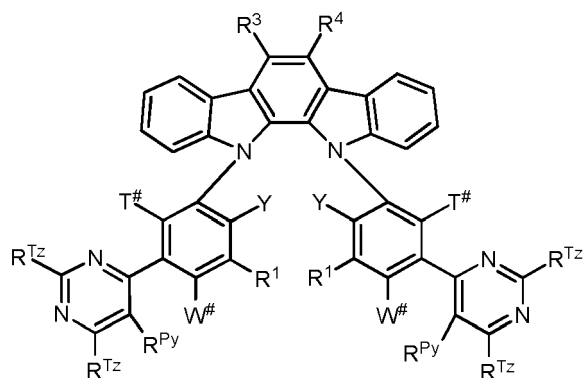
Formula X
