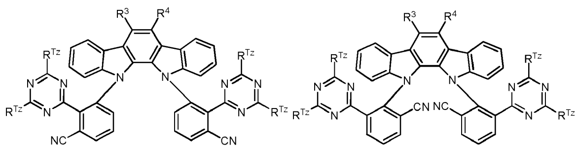
Formula IIIc
