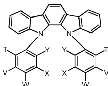
Formula III-AAA
