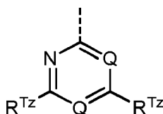
Formula Py
