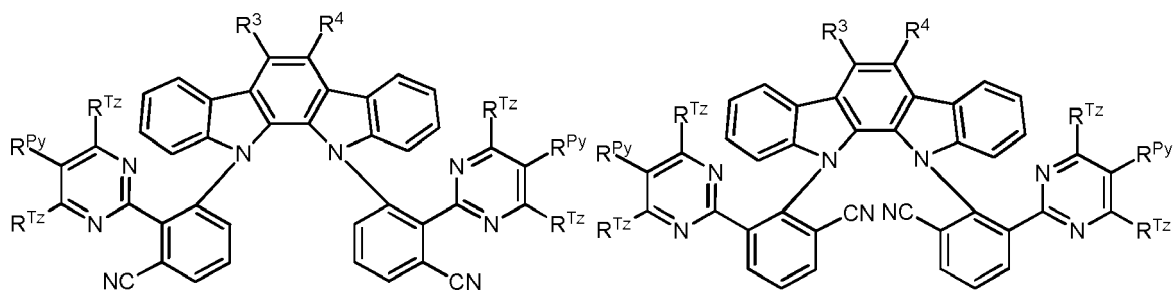
Formula Vc
