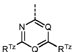
Formula Py
