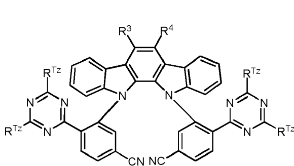
Formula IIIa
