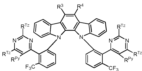
Formula IVg
