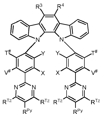
Formula VIII
