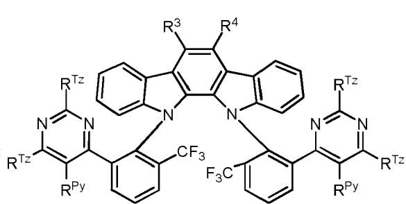
Formula IVh
