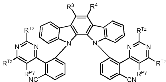
Formula IVc
