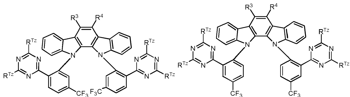
Formula IIIe
