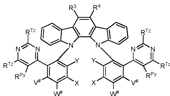
Formula IV
