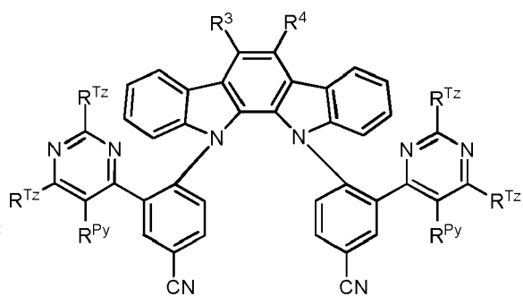
Formula IVb
