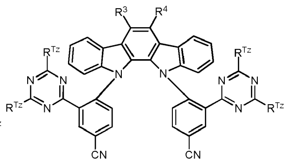
Formula IIIb
