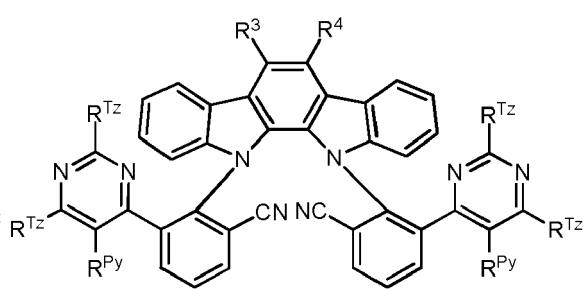
Formula IVd
