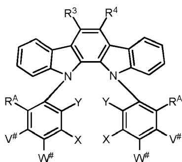
Formula III-Y
