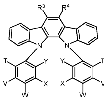
Formula I
