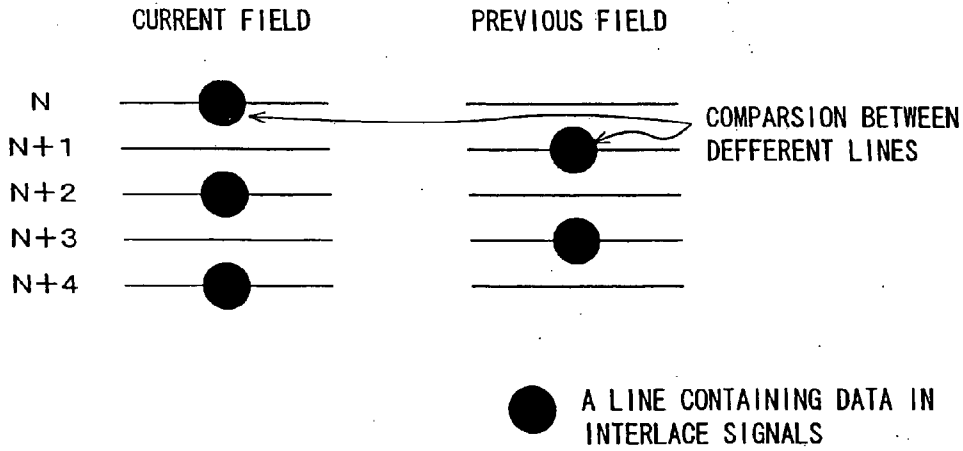
FIG. 17 PRIOR ART
