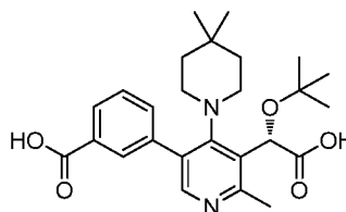
Example 147
