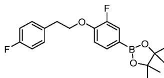
Intermediate 62
