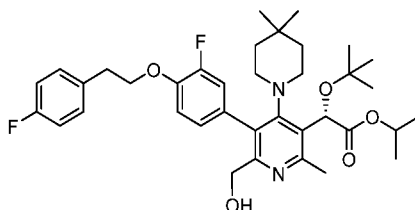
Intermediate 143
