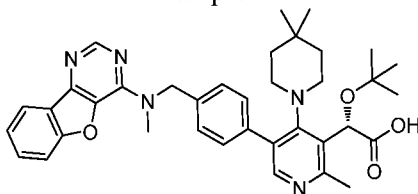
Example 20
