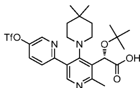
Intermediate 263
