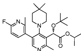
Intermediate 232
