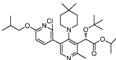
Intermediate 255
