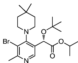
Intermediate 32
