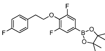
Intermediate 75
