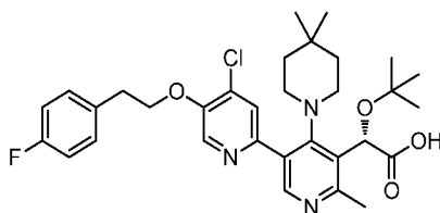
Example 447
