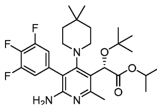
Intermediate 120
