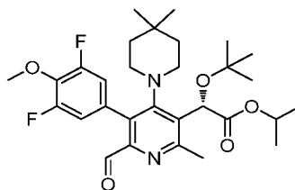
Intermediate 126
