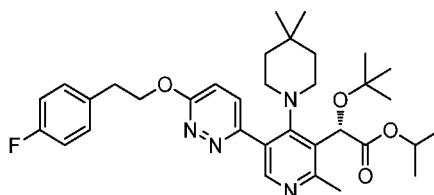
Intermediate 112
