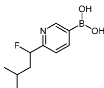
(6-(1-Fluoro-3-methylbutyl)pyridin-3-yl)boronic acid:
