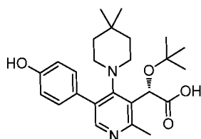
Intermediate 20
