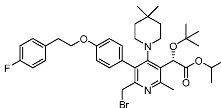
Intermediate 113
