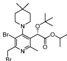
Intermediate 5
