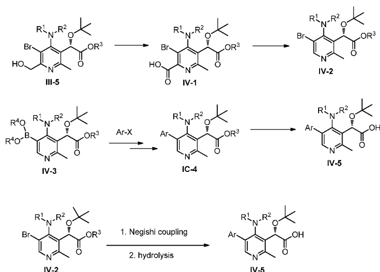
Scheme IV
