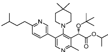
Intermediate 241
