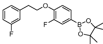
Intermediate 83
