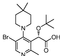
Intermediate 10
