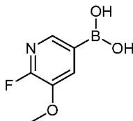
Intermediate 215
