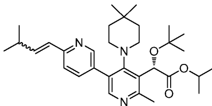
Intermediate 240
