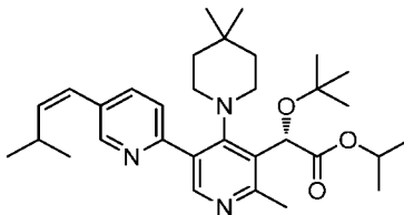
Intermediate 181
