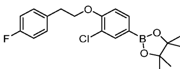
Intermediate 87
