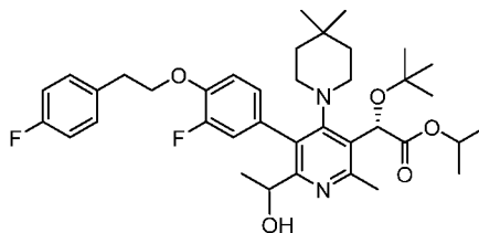
Intermediate 146
