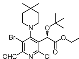
Intermediate 38
