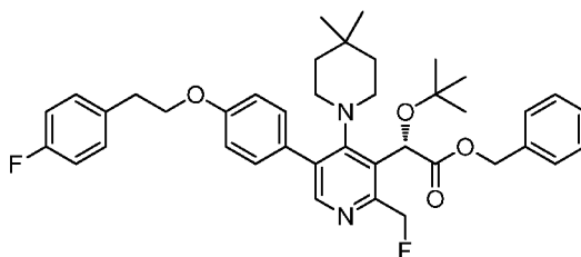
Intermediate 101
