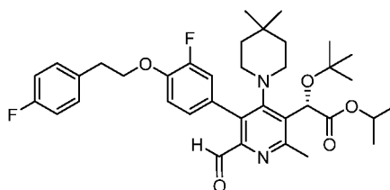
Intermediate 144
