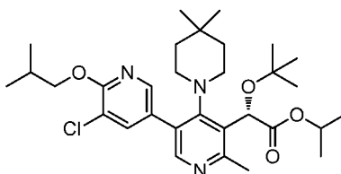
Intermediate 231
