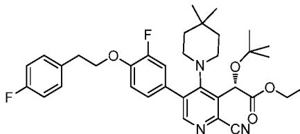
Intermediate 136
