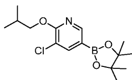
Intermediate 230
