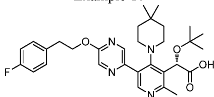
Example 16
