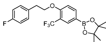
Intermediate 91
