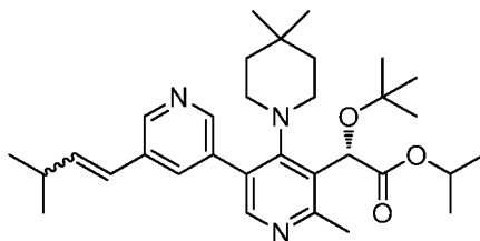
Intermediate 236
