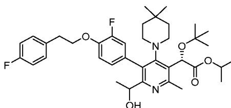
Intermediate 145
