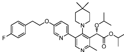
Intermediate 177
