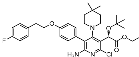
Intermediate 129
