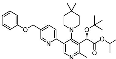
Intermediate 179
