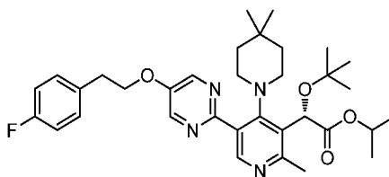
Intermediate 106
