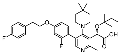
Example 450
