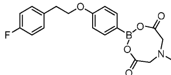
Intermediate 58
