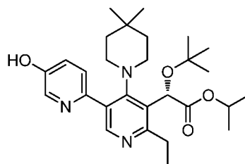
Intermediate 198
