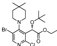
Intermediate 37
