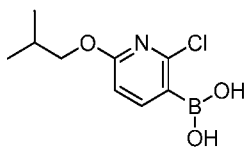
Intermediate 254
