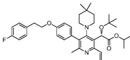
Intermediate 96
