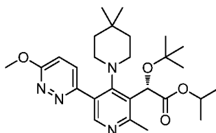
Intermediate 108
