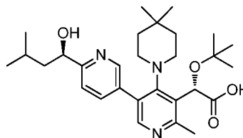
Example 433
