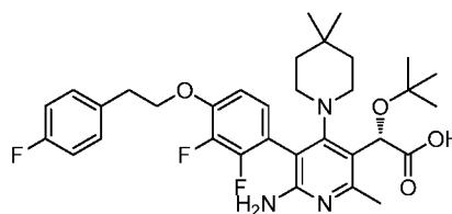
Example 71
