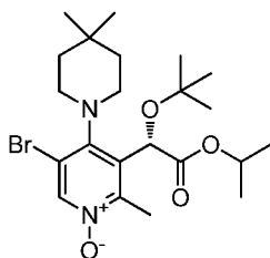
Intermediate 15
