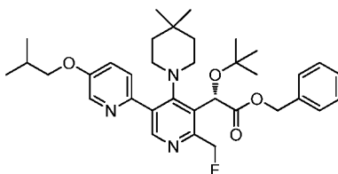
Intermediate 196
