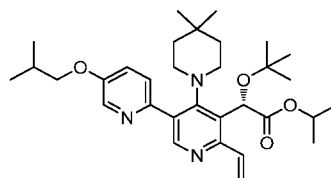
Intermediate 194
