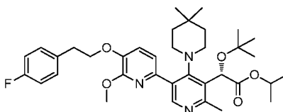
Intermediate 162
