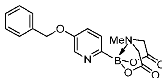
Intermediate 95
