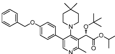
Intermediate 150
