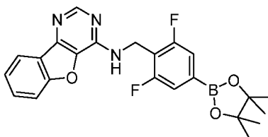
Intermediate 55
