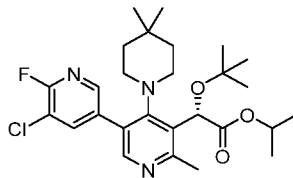
Intermediate 139
