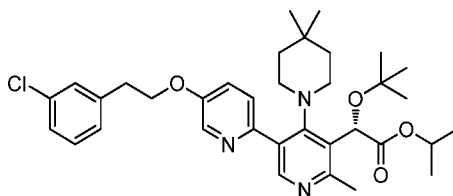
Intermediate 205
