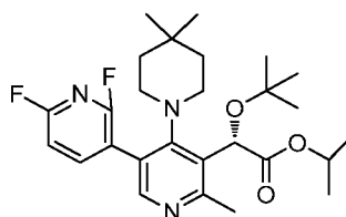
Intermediate 258
