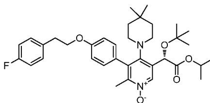
Intermediate 99
