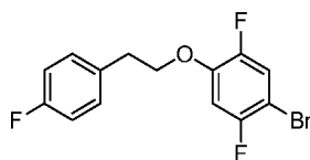
Intermediate 69
