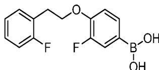
Intermediate 73
