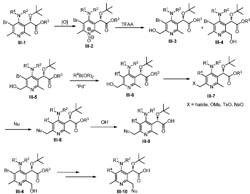
Scheme III
