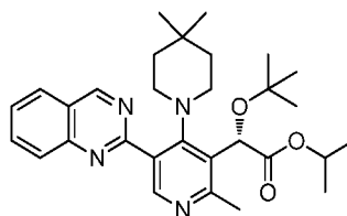
Intermediate 168
