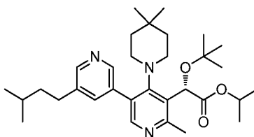
Intermediate 237
