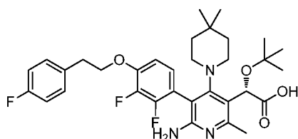
Example 70
