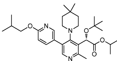
Intermediate 214
