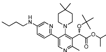
Intermediate 264
