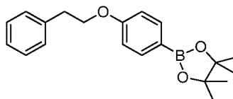
Intermediate 93
