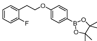
Intermediate 81
