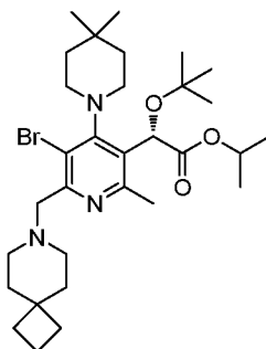
Intermediate 125
