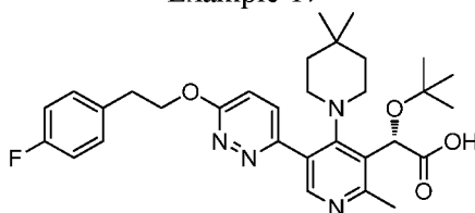
Example 17
