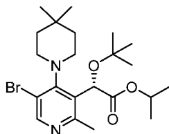
Intermediate 9
