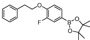
2-(3-Fluoro-4-phenethoxyphenyl)-4,4,5,5-tetramethyl-1,3,2-dioxaborolane:
