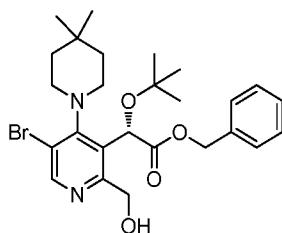
Intermediate 13
