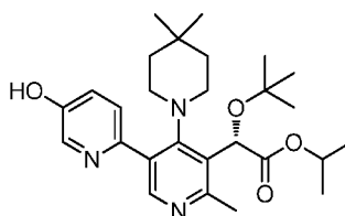
Intermediate 149
