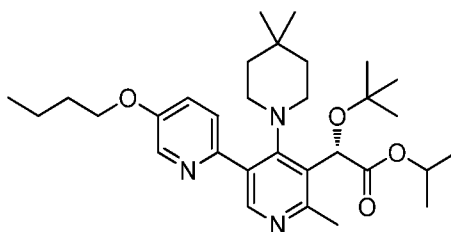
Intermediate 203
