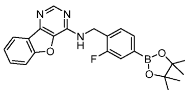
Intermediate 53
