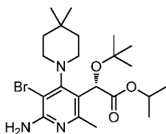
Intermediate 8
