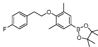
Intermediate 79
