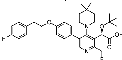
Example 7
