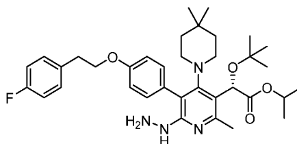
Intermediate 121
