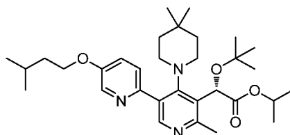
Intermediate 208
