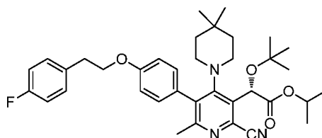
Intermediate 100
