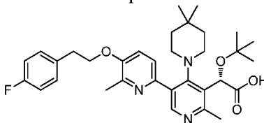
Example 232
