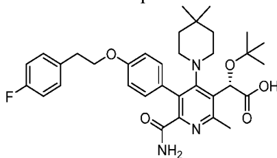
Example 13
