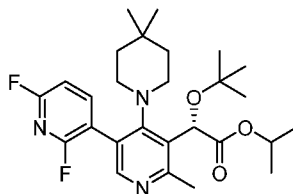
Intermediate 142
