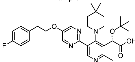
Example 14
