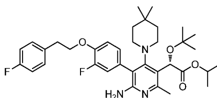
Intermediate 117
