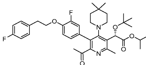
Intermediate 147
