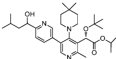
Intermediate 257
