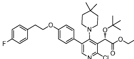
Intermediate 127
