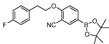
Intermediate 89
