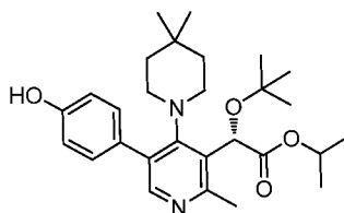
Intermediate 19
