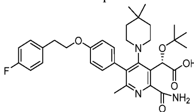
Example 6
