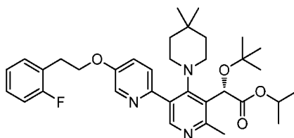
Intermediate 206
