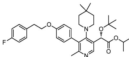
Intermediate 98
