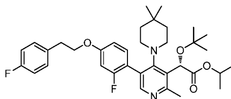
Intermediate 123
