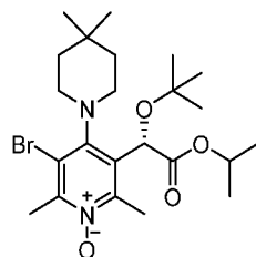
Intermediate 2
