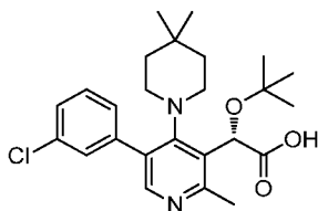
Example 143
