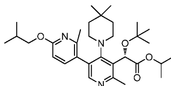
Intermediate 233
