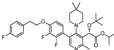
Intermediate 124
