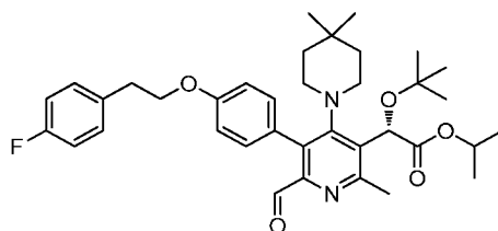
Intermediate 103
