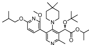
Intermediate 225
