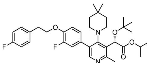
Intermediate 122
