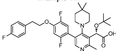
Example 125
