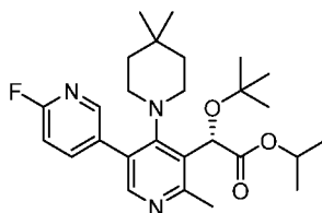
Intermediate 107
