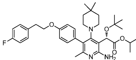
Intermediate 97
