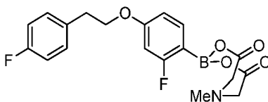
Intermediate 65
