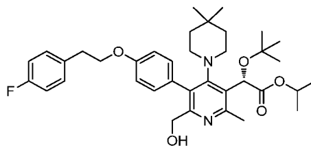
Intermediate 102
