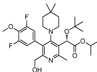
Intermediate 109
