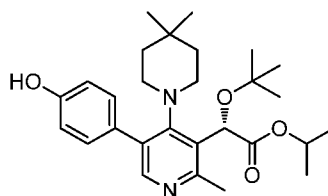
Intermediate 151
