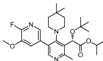
Intermediate 216
