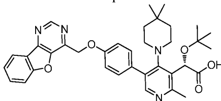
Example 19
