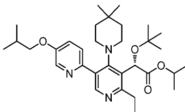
Intermediate 195
