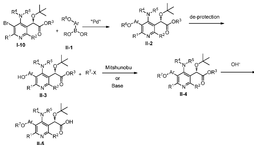
Scheme II
