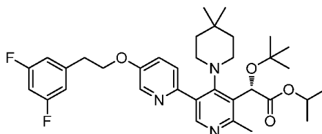
Intermediate 207
