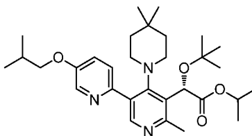
Intermediate 204
