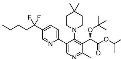
Intermediate 191
