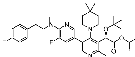
Intermediate 228
