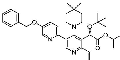
Intermediate 197
