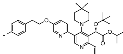
Intermediate 174
