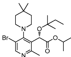
Intermediate 18
