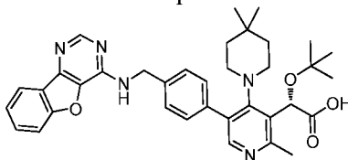
Example 21
