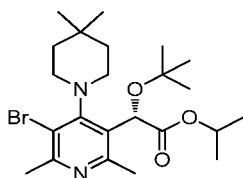
Intermediate 1
