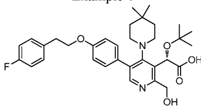
Example 8
