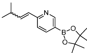
Intermediate 239
