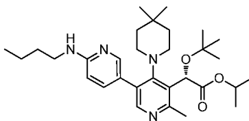
Intermediate 262
