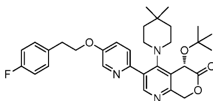
Intermediate 171
