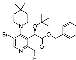
Intermediate 14
