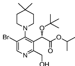
Intermediate 16
