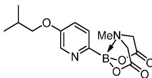
Intermediate 193
