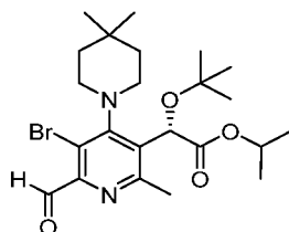
Intermediate 6
