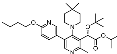
Intermediate 248
