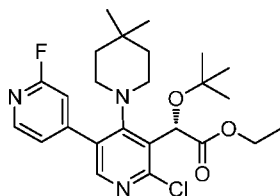
Intermediate 135
