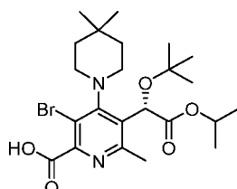
Intermediate 7
