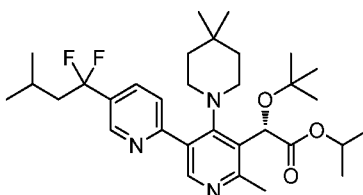
Intermediate 185
