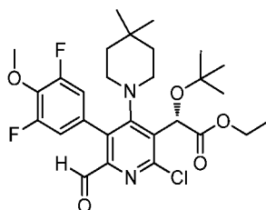
Intermediate 128
