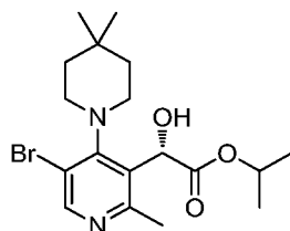
Intermediate 17
