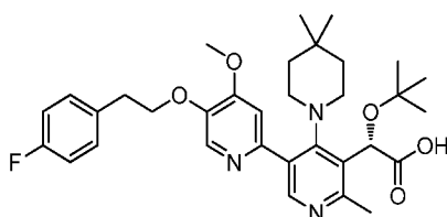
Example 449
