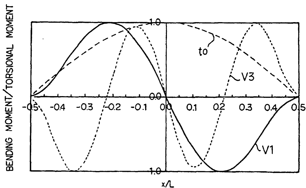
MEASURING POINT IN LONGITUDINAL DIRECTION Fig. 11
