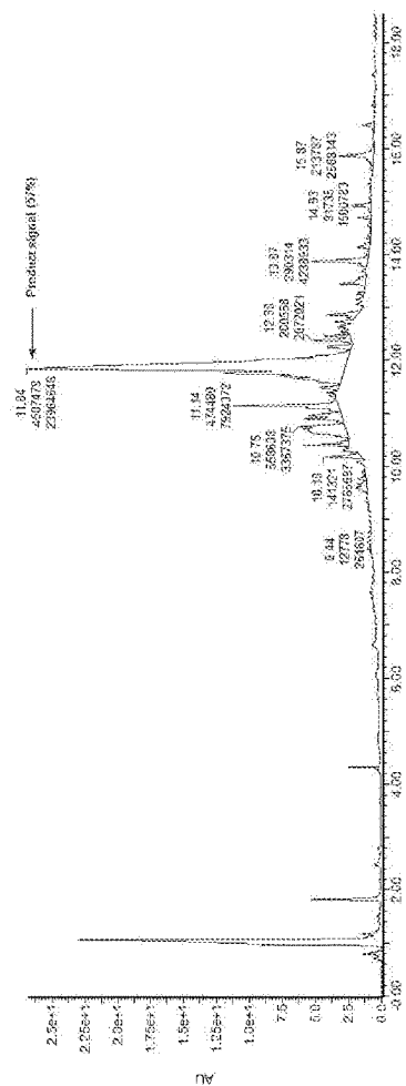
Figure 3 UPLC Chromatogram – Table 1, Entry 5
