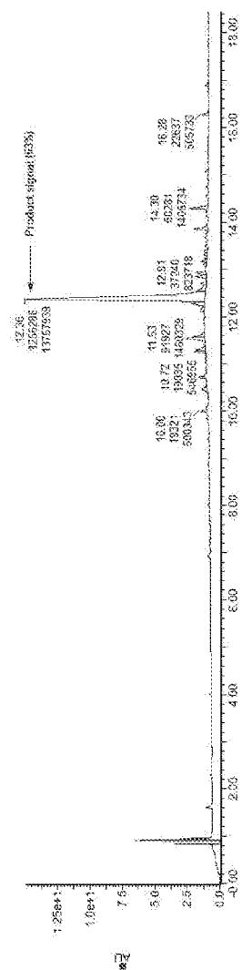
Figure 4 UPLC Chromatogram – Table 2, Entry 3
