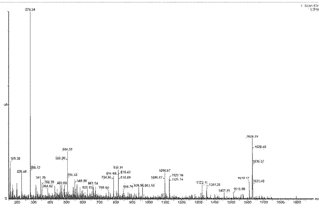
Figure 15 MS Data – Table 7, Entry 2
