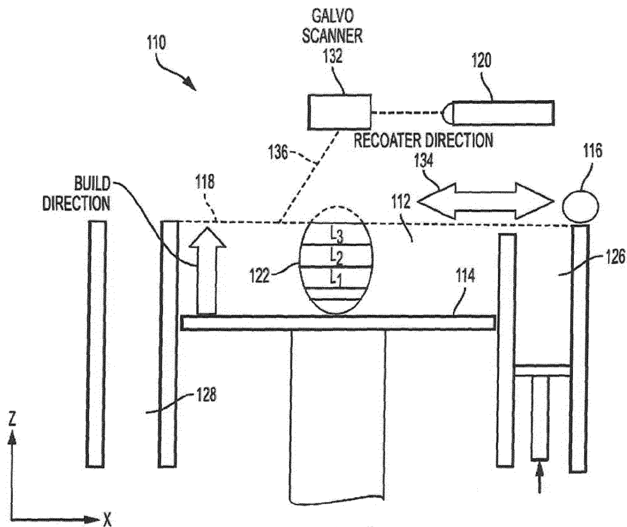
FIG. 1 PRIOR ART
