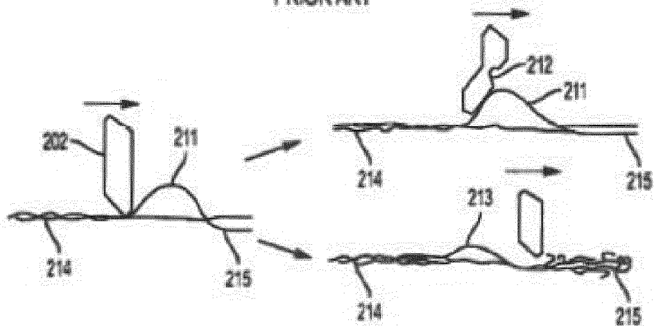
FIG. 2C PRIOR ART
