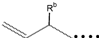
3-alkyl vinyl end group
