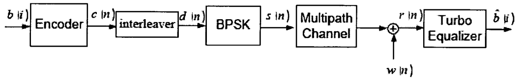
Fig. 6. Transmitter and receiver chain.
