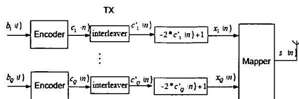
Fig. 1. Transmitter chain.
