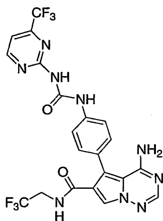
4-amino-N-cyclopropyl-5-{4-[[[4-(trifluoromethyl)pyrimidin-2-yl]amino]carbonyl]amino}phenyl}pyrrolo[2,1-f][1,2,4]triazine-6-carboxamide
