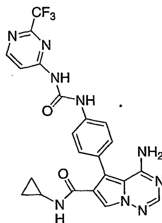
4-amino-N-(2,2,2-trifluoroethyl)-5-{4-[[[3-(trifluoromethoxy)phenyl]amino]carbonyl]amino}phenyl}pyrrolo[2,1-f][1,2,4]triazine-6-carboxamide
