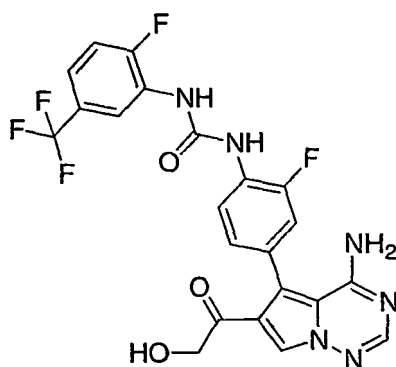
N-{4-[4-amino-6-(1,3-thiazol-5-yl)pyrrolo[2,1-f][1,2,4]triazin-5-yl]phenyl}-N'-[4-(trifluoromethyl)pyridin-2-yl]urea
