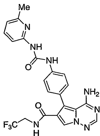
4-amino-N-cyclopropyl-5-[4-({[(6-methylpyridin-2-yl)amino]carbonyl}amino)phenyl]pyrrolo[2,1-f][1,2,4]triazine-6-carboxamide
