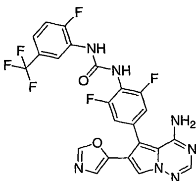
N-{4-[4-amino-6-(1,3-oxazol-5-yl)pyrrolo[2,1-f][1,2,4]triazin-5-yl]-2-chlorophenyl}-N'-[4-(trifluoromethyl)pyridin-2-yl]urea
