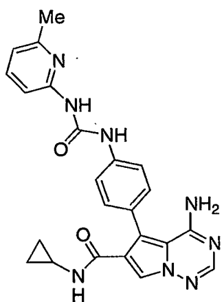
4-amino-5-[4-({[3-(3-ethylphenoxy)phenyl]amino}carbonyl}amino)phenyl]-N-(2,2,2-trifluoroethyl)pyrrolo[2,1-f][1,2,4]triazine-6-carboxamide
