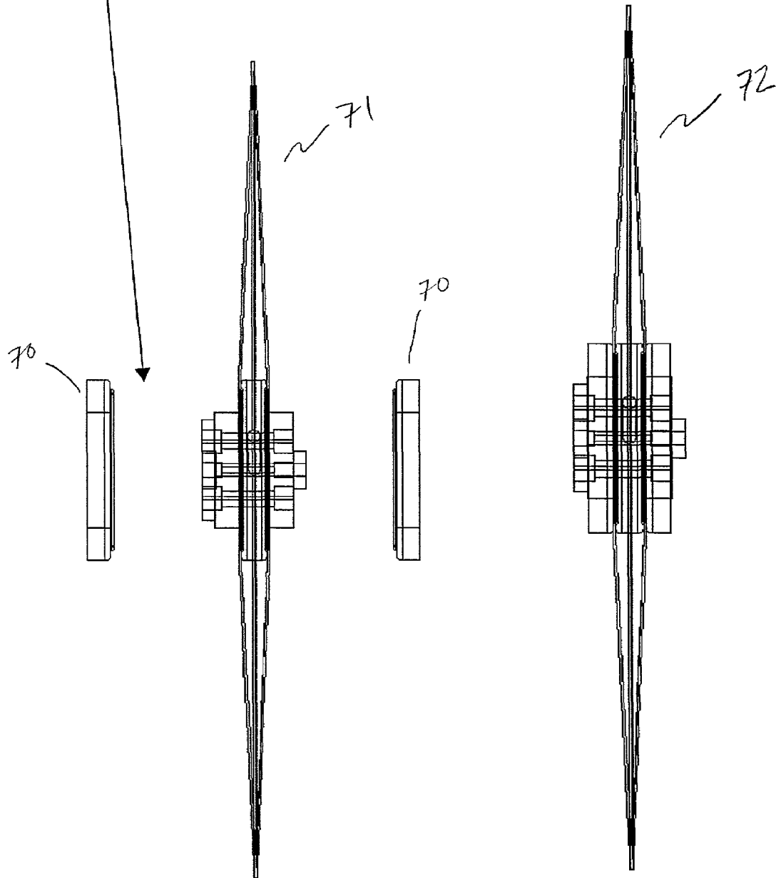
FIGURE 7 PROCESSING BAG ASSEMBLY
