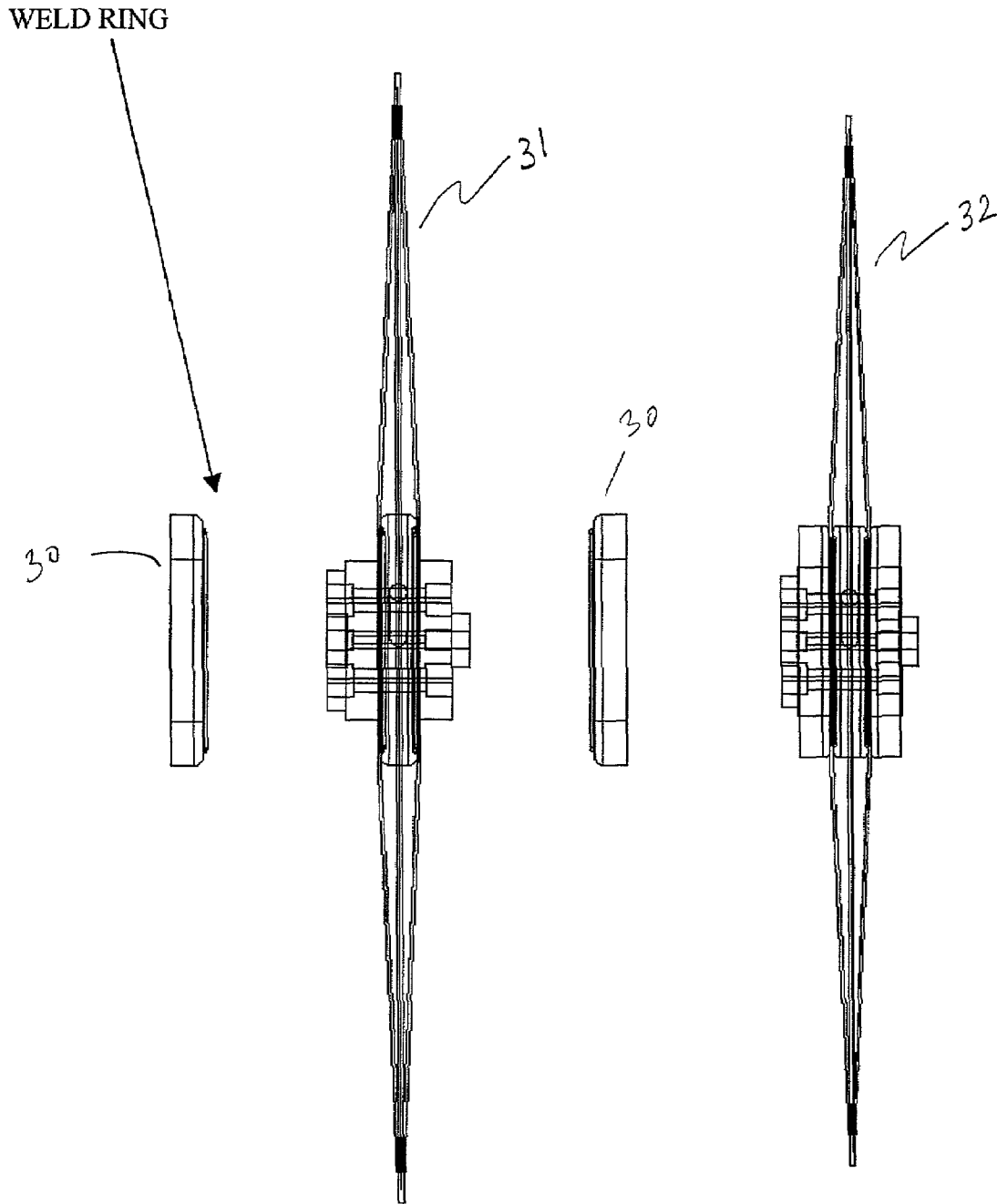
FIGURE 3 EXPRESSOR BAG ASSEMBLY
