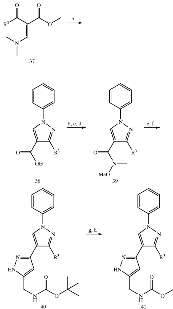
Scheme VII
