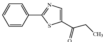
1-(2-Phenyl-thiazol-5-yl)-propan-1-one
