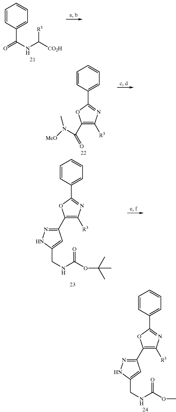
Scheme V
