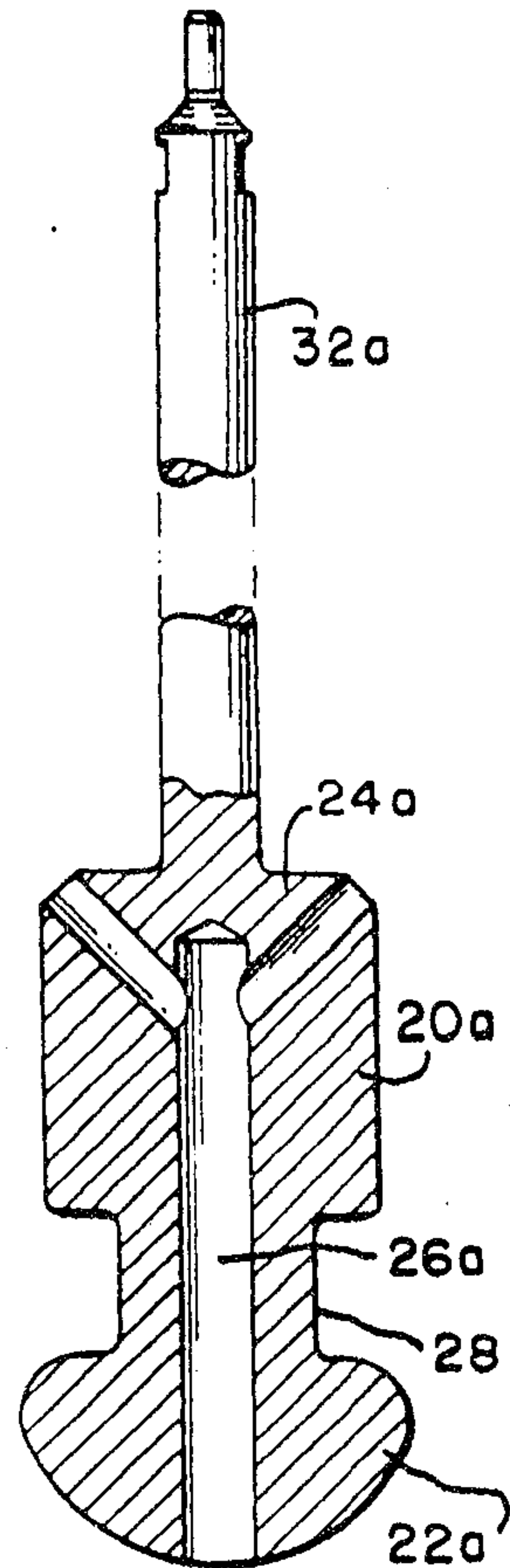
FIG. 2 (PRIOR ART)
