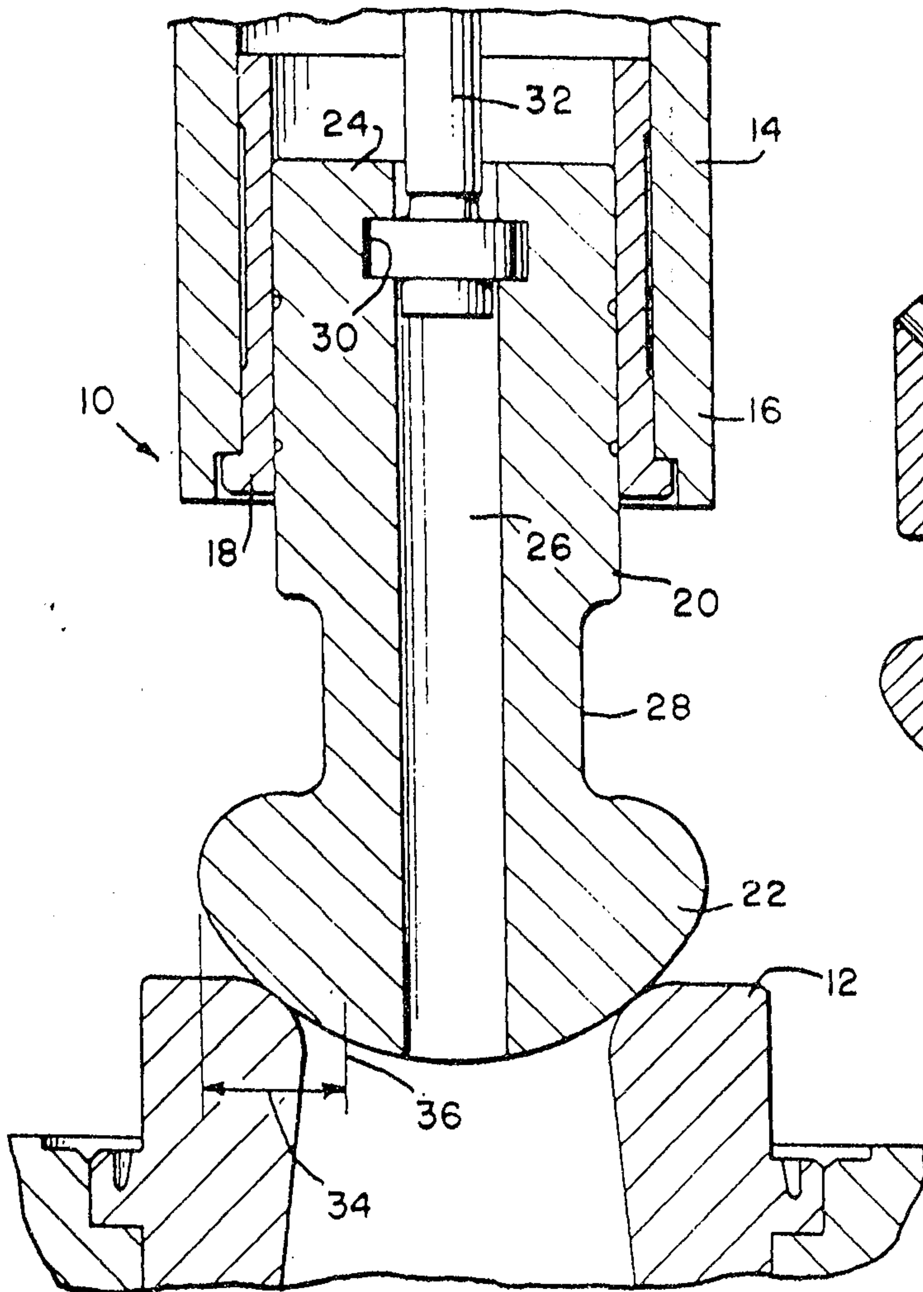
FIG. 1 (PRIOR ART)
