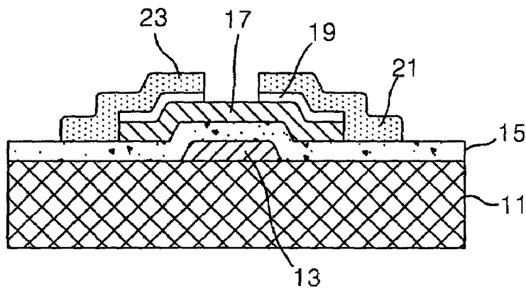
FIG. 1C CONVENTIONAL ART
