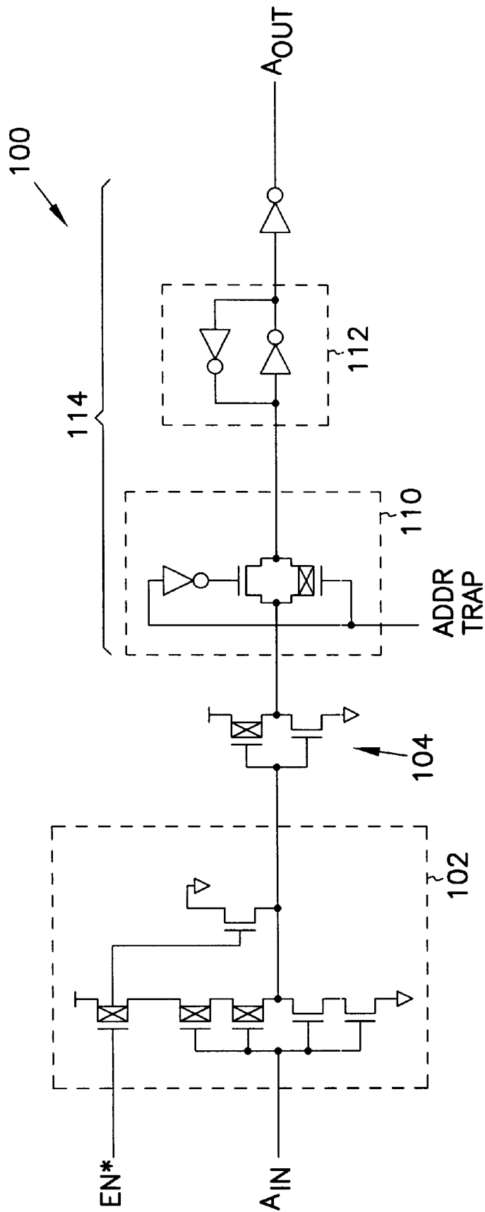
FIG. 1 (PRIOR ART)
