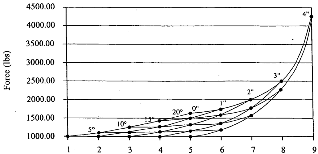
Carpet Plot - H-Car
