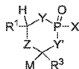
[0051] (Ic)
