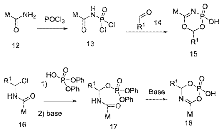
Scheme III
