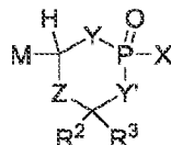
[0038] (Ib)
