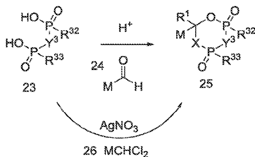
[0393] Scheme V
