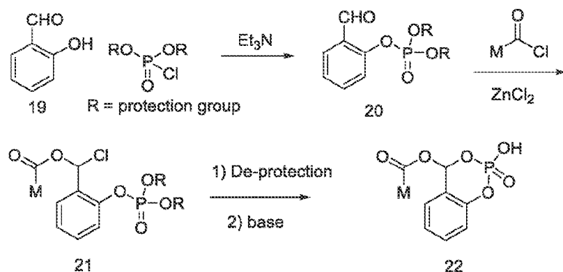
Scheme IV
