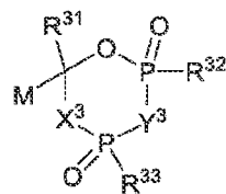
[0089] (III)
