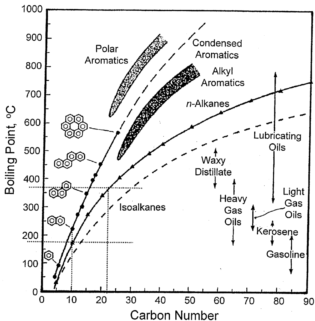
Relationship of boiling point to carbon number
