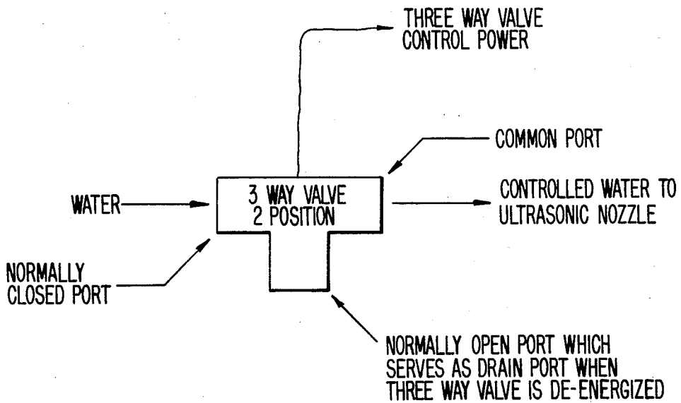
FIG. 3. (PRIOR ART)
