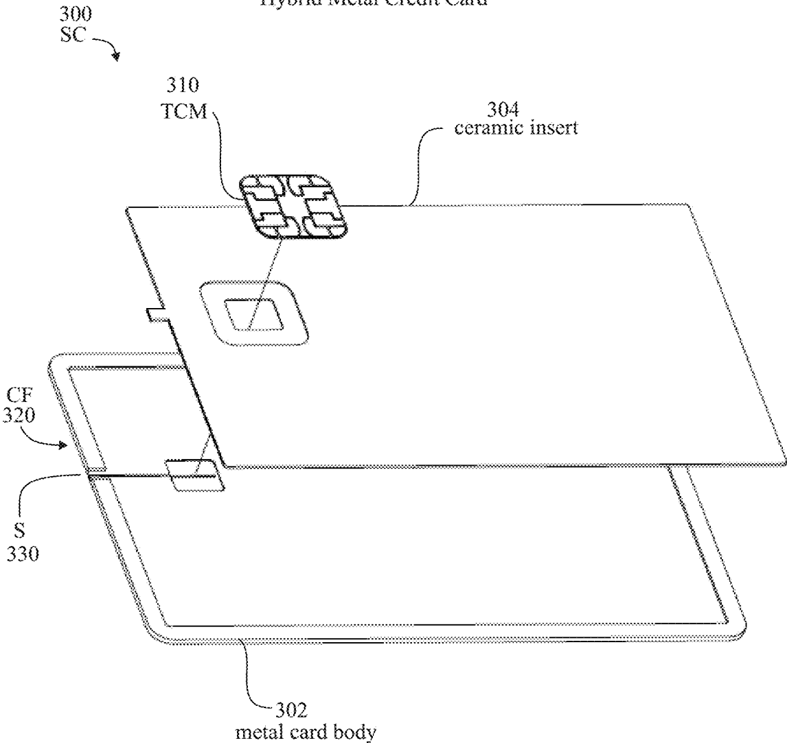
FIG. 3D Hybrid Metal Credit Card
