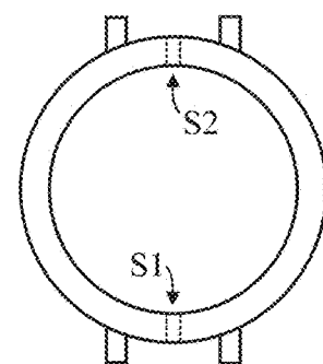
FIG. 10D concealed slits
