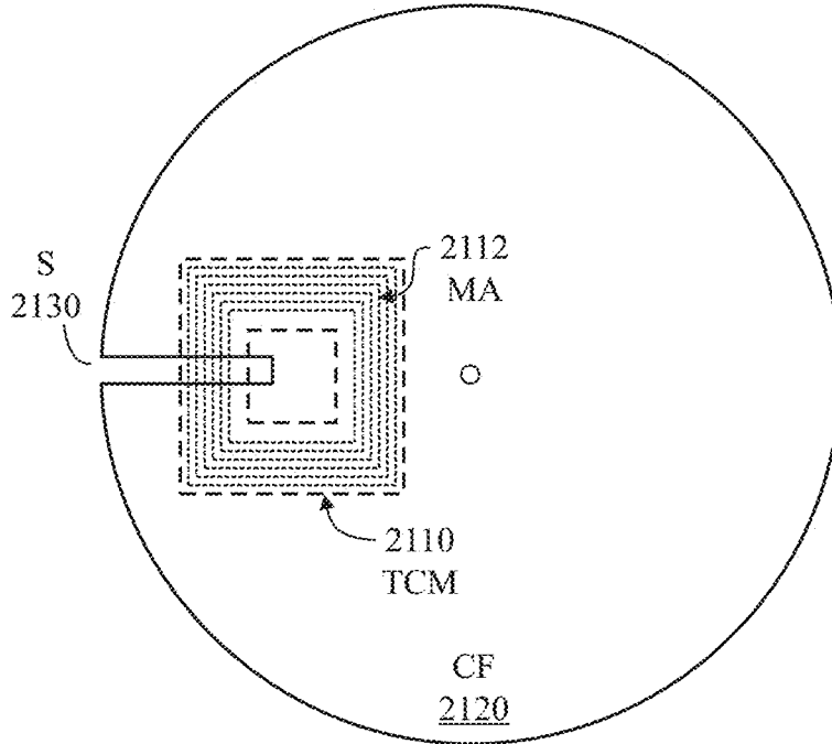
FIG. 21A one CF, one TCM, enabled
