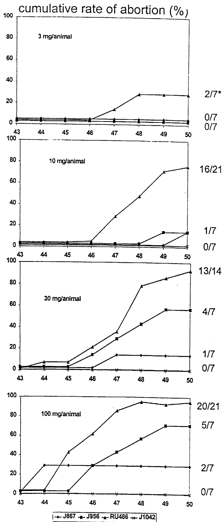
Figure 2: Cumulative rate of abortion until day 50 in guinea pigs treatment on days 43 and 44 of pregnancy by s.c. injection. (##) = rate of abortion
